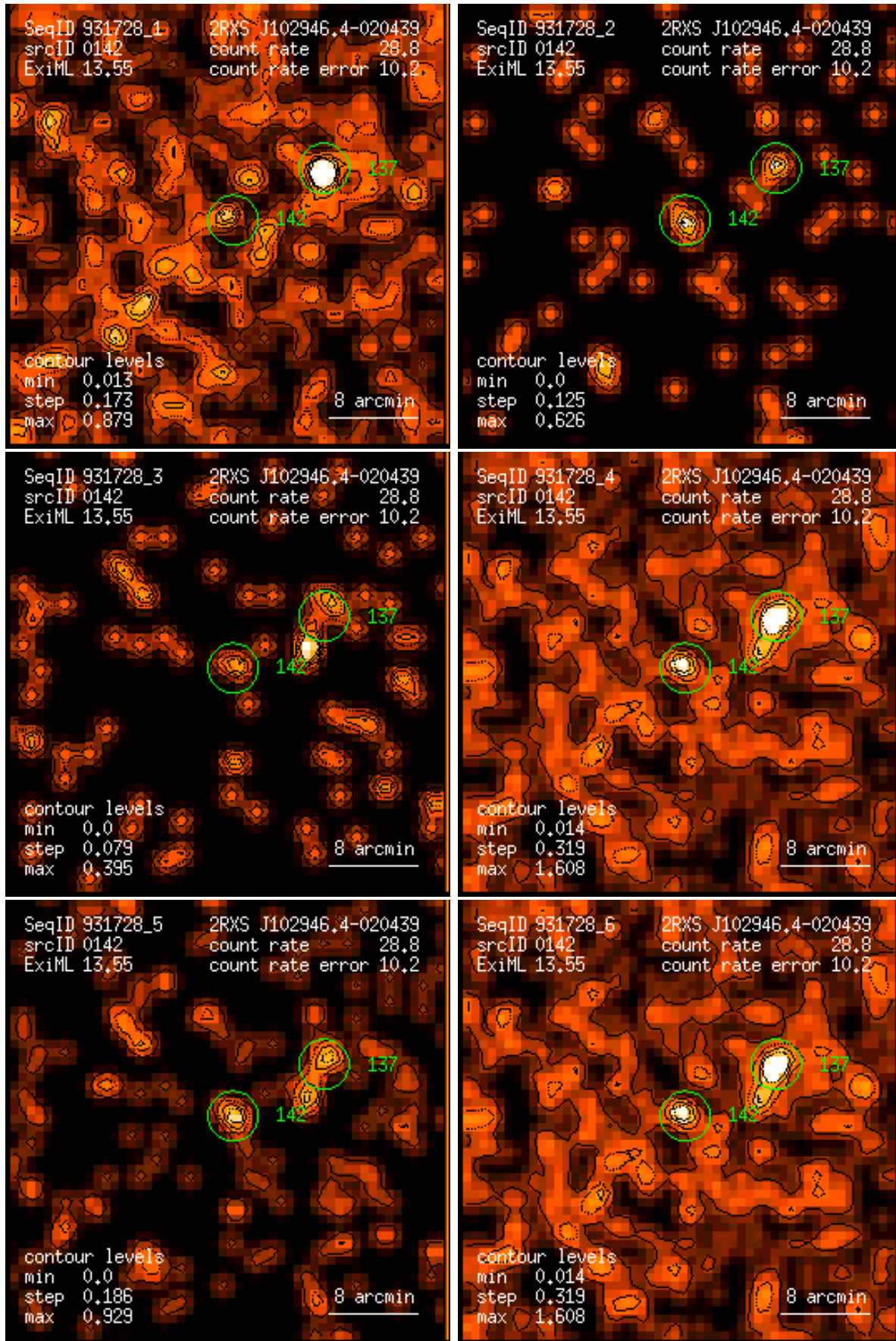
Figure 142: RASS 931728: detection 0142: band rate images, Gaussian filter: (1) PSPC channels 11 – 41, (2) 52 – 90, (3) 91 – 201, (4) 11 – 235, (5) 52 – 201, (6) 11 – 201. Broad band rates in counts/ks. Band rate contour levels in counts/ks/arcmin 2 .
