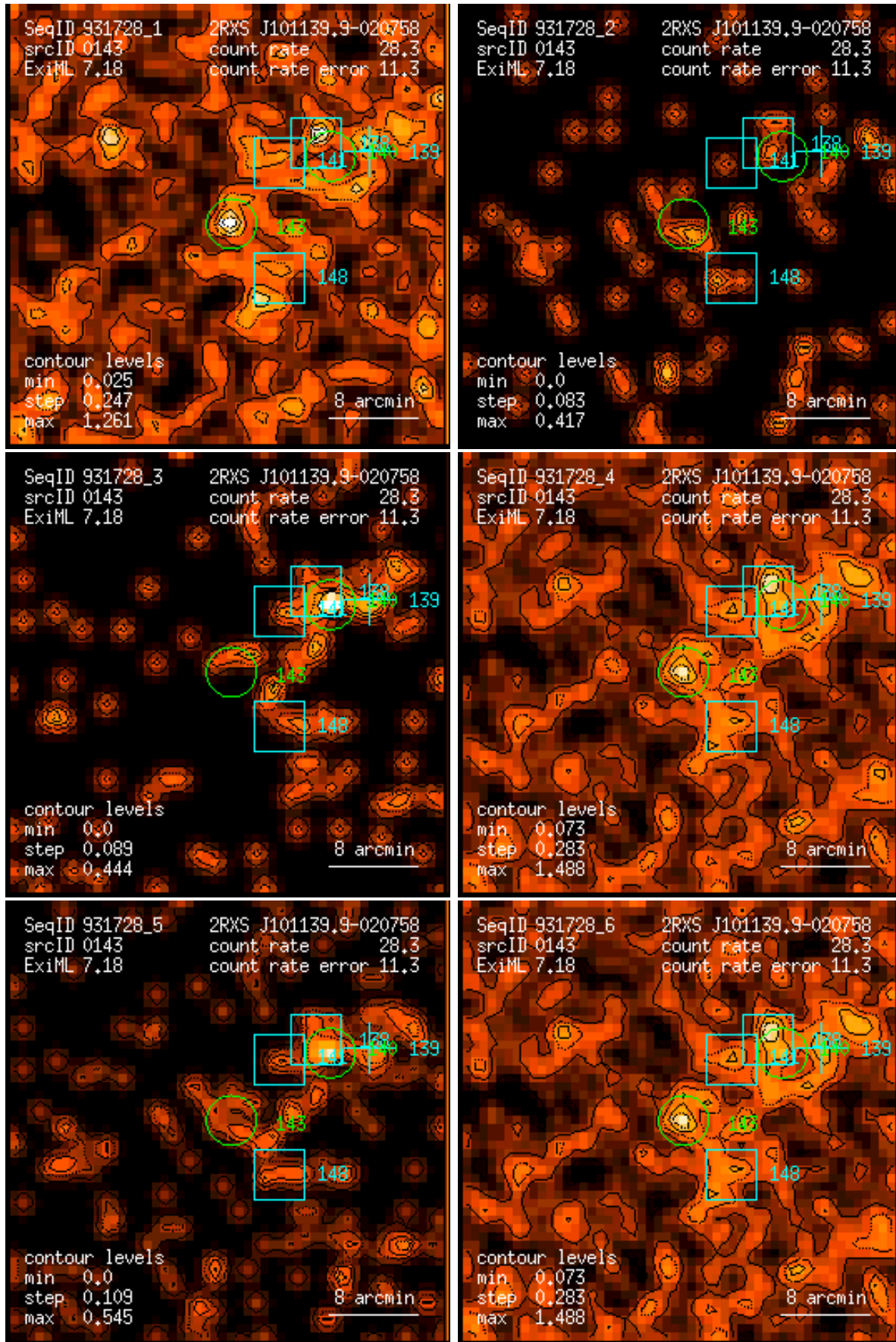
Figure 143: RASS 931728: detection 0143: band rate images, Gaussian filter: (1) PSPC channels 11 – 41, (2) 52 – 90, (3) 91 – 201, (4) 11 – 235, (5) 52 – 201, (6) 11 – 201. Broad band rates in counts/ks. Band rate contour levels in counts/ks/arcmin 2 .
