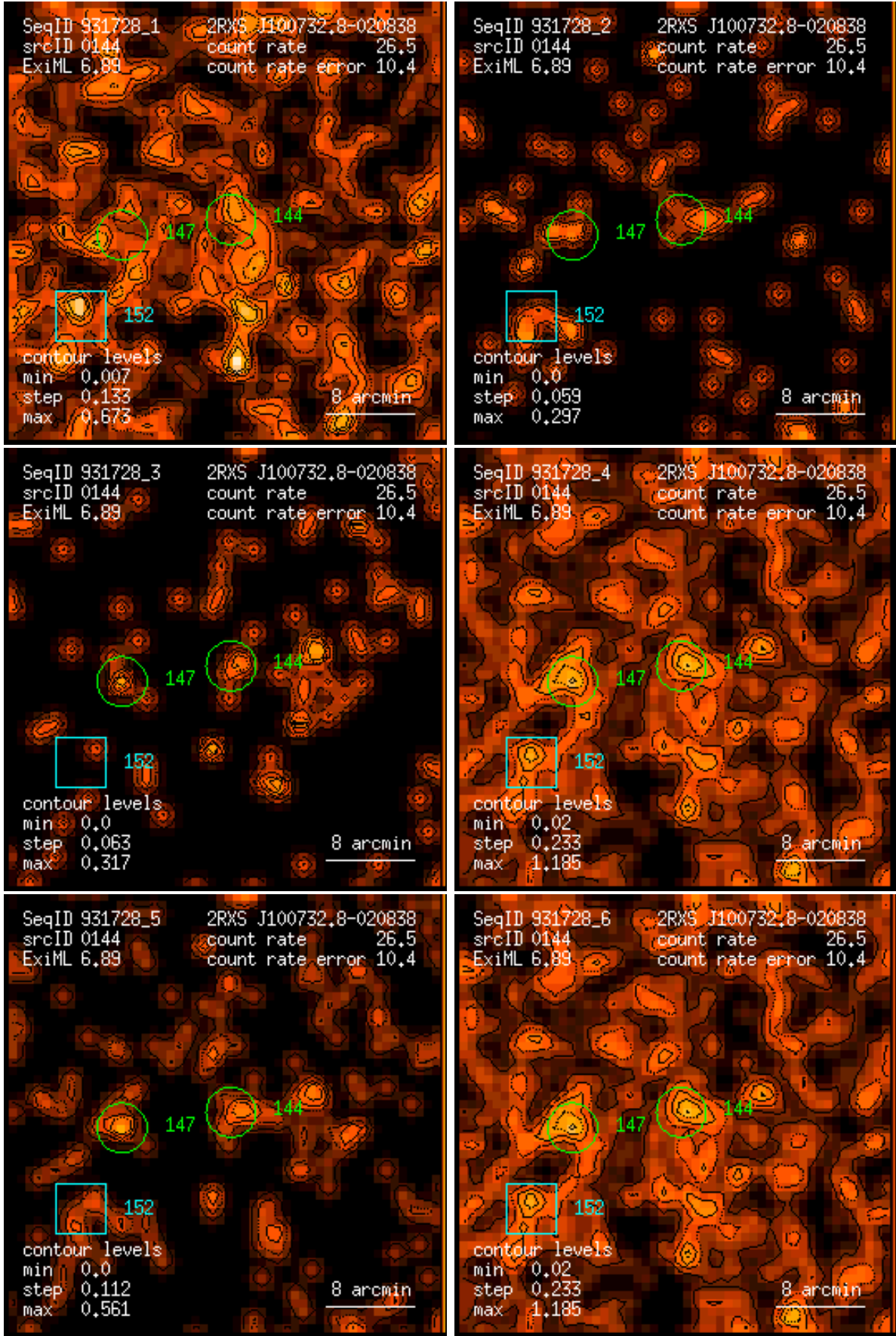
Figure 144: RASS 931728: detection 0144: band rate images, Gaussian filter: (1) PSPC channels 11 – 41, (2) 52 – 90, (3) 91 – 201, (4) 11 – 235, (5) 52 – 201, (6) 11 – 201. Broad band rates in counts/ks. Band rate contour levels in counts/ks/arcmin 2 .
