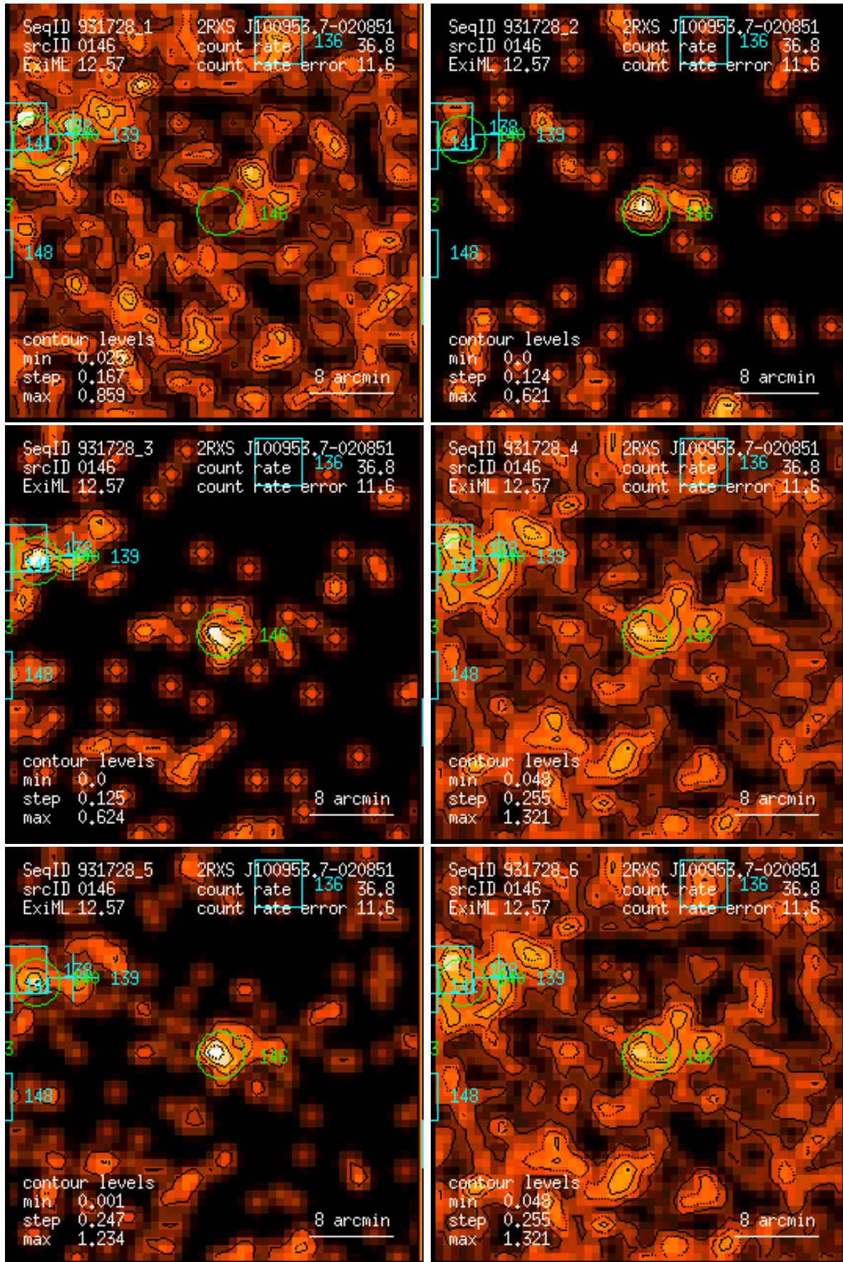
Figure 146: RASS 931728: detection 0146: band rate images, Gaussian filter: (1) PSPC channels 11 – 41, (2) 52 – 90, (3) 91 – 201, (4) 11 – 235, (5) 52 – 201, (6) 11 – 201. Broad band rates in counts/ks. Band rate contour levels in counts/ks/arcmin 2 .
