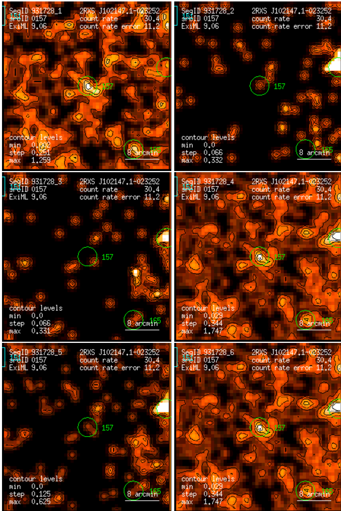
Figure 157: RASS 931728: detection 0157: band rate images, Gaussian filter: (1) PSPC channels 11 – 41, (2) 52 – 90, (3) 91 – 201, (4) 11 – 235, (5) 52 – 201, (6) 11 – 201. Broad band rates in counts/ks. Band rate contour levels in counts/ks/arcmin 2 .
