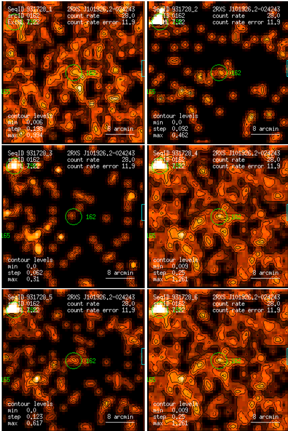
Figure 162: RASS 931728: detection 0162: band rate images, Gaussian filter: (1) PSPC channels 11 – 41, (2) 52 – 90, (3) 91 – 201, (4) 11 – 235, (5) 52 – 201, (6) 11 – 201. Broad band rates in counts/ks. Band rate contour levels in counts/ks/arcmin 2 .
