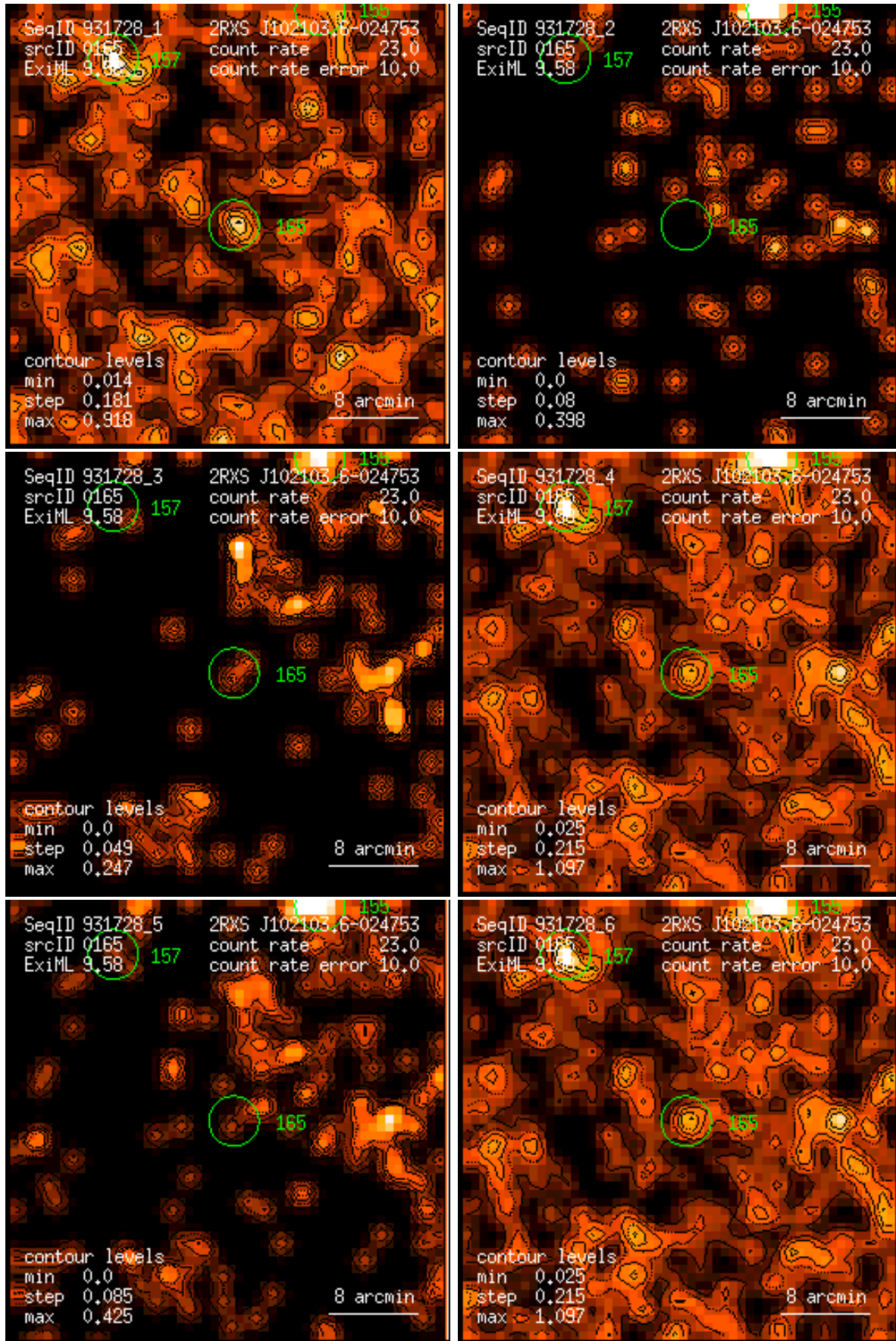
Figure 165: RASS 931728: detection 0165: band rate images, Gaussian filter: (1) PSPC channels 11 – 41, (2) 52 – 90, (3) 91 – 201, (4) 11 – 235, (5) 52 – 201, (6) 11 – 201. Broad band rates in counts/ks. Band rate contour levels in counts/ks/arcmin 2 .
