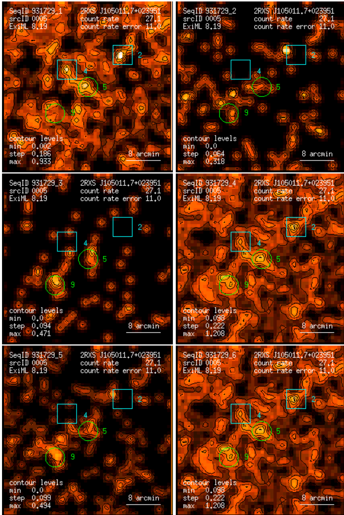
Figure 5: RASS 931729: detection 0005: band rate images, Gaussian filter: (1) PSPC channels 11 – 41, (2) 52 – 90, (3) 91 – 201, (4) 11 – 235, (5) 52 – 201, (6) 11 – 201. Broad band rates in counts/ks. Band rate contour levels in counts/ks/arcmin 2 .
