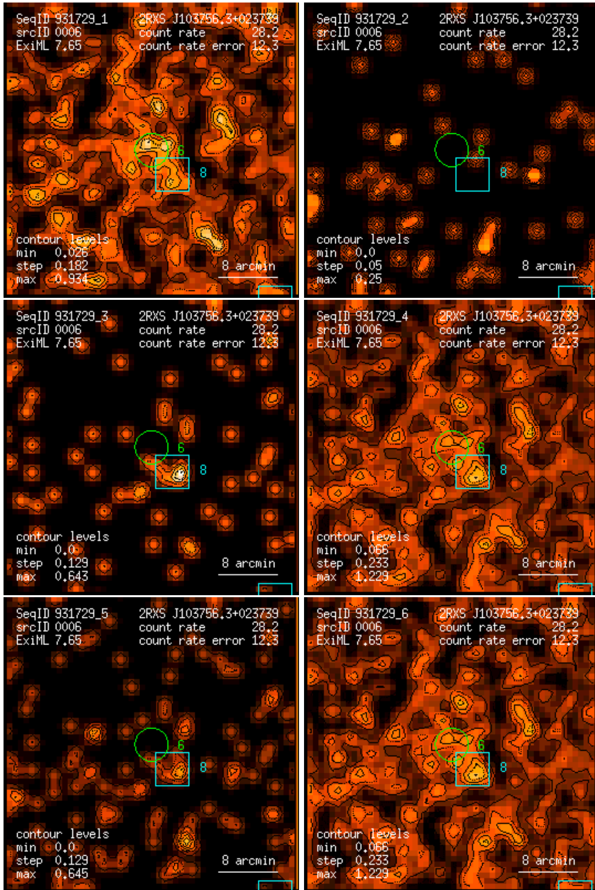
Figure 6: RASS 931729: detection 0006: band rate images, Gaussian filter: (1) PSPC channels 11 – 41, (2) 52 – 90, (3) 91 – 201, (4) 11 – 235, (5) 52 – 201, (6) 11 – 201. Broad band rates in counts/ks. Band rate contour levels in counts/ks/arcmin 2 .
