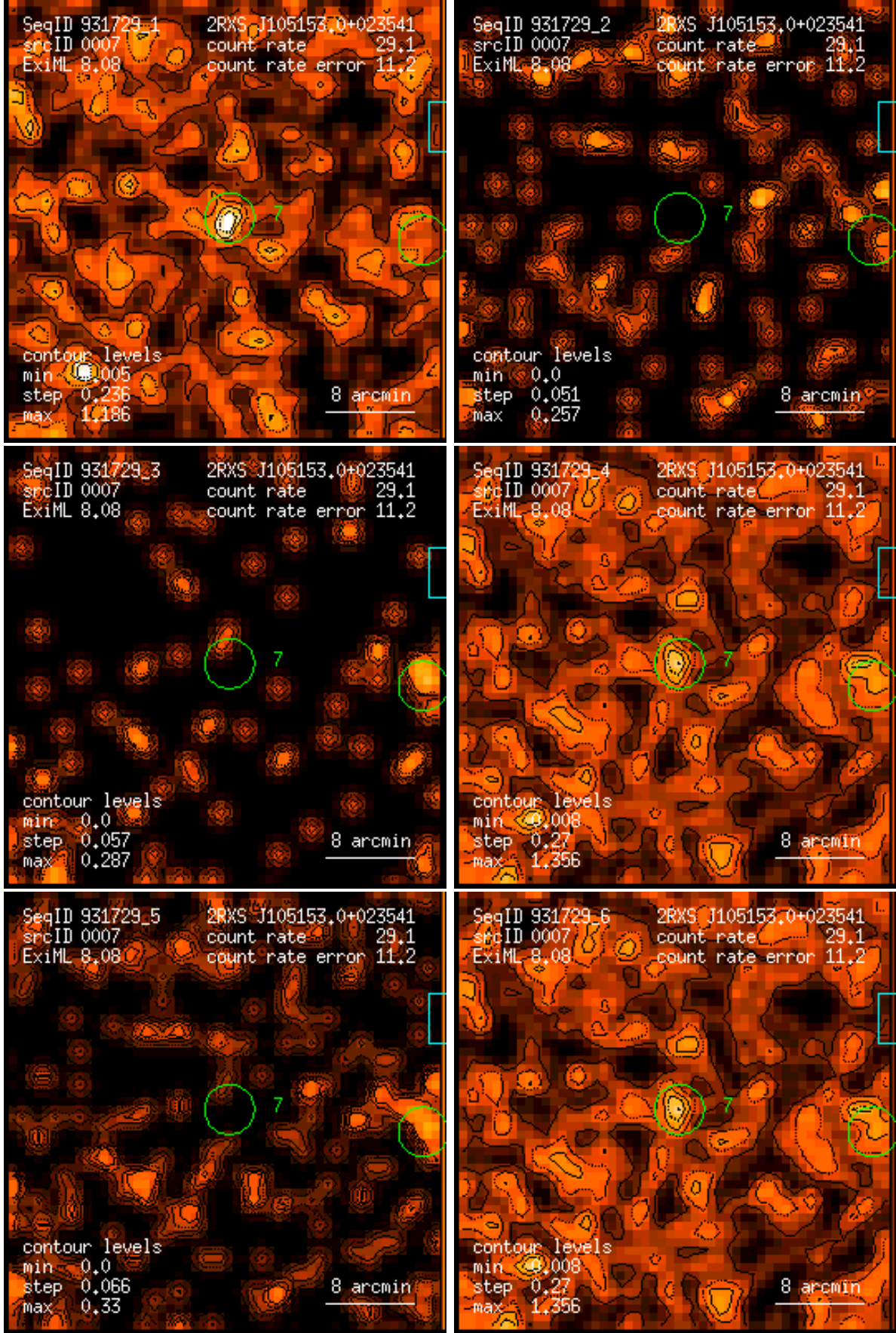
Figure 7: RASS 931729: detection 0007: band rate images, Gaussian filter: (1) PSPC channels 11 – 41, (2) 52 – 90, (3) 91 – 201, (4) 11 – 235, (5) 52 – 201, (6) 11 – 201. Broad band rates in counts/ks. Band rate contour levels in counts/ks/arcmin 2 .
