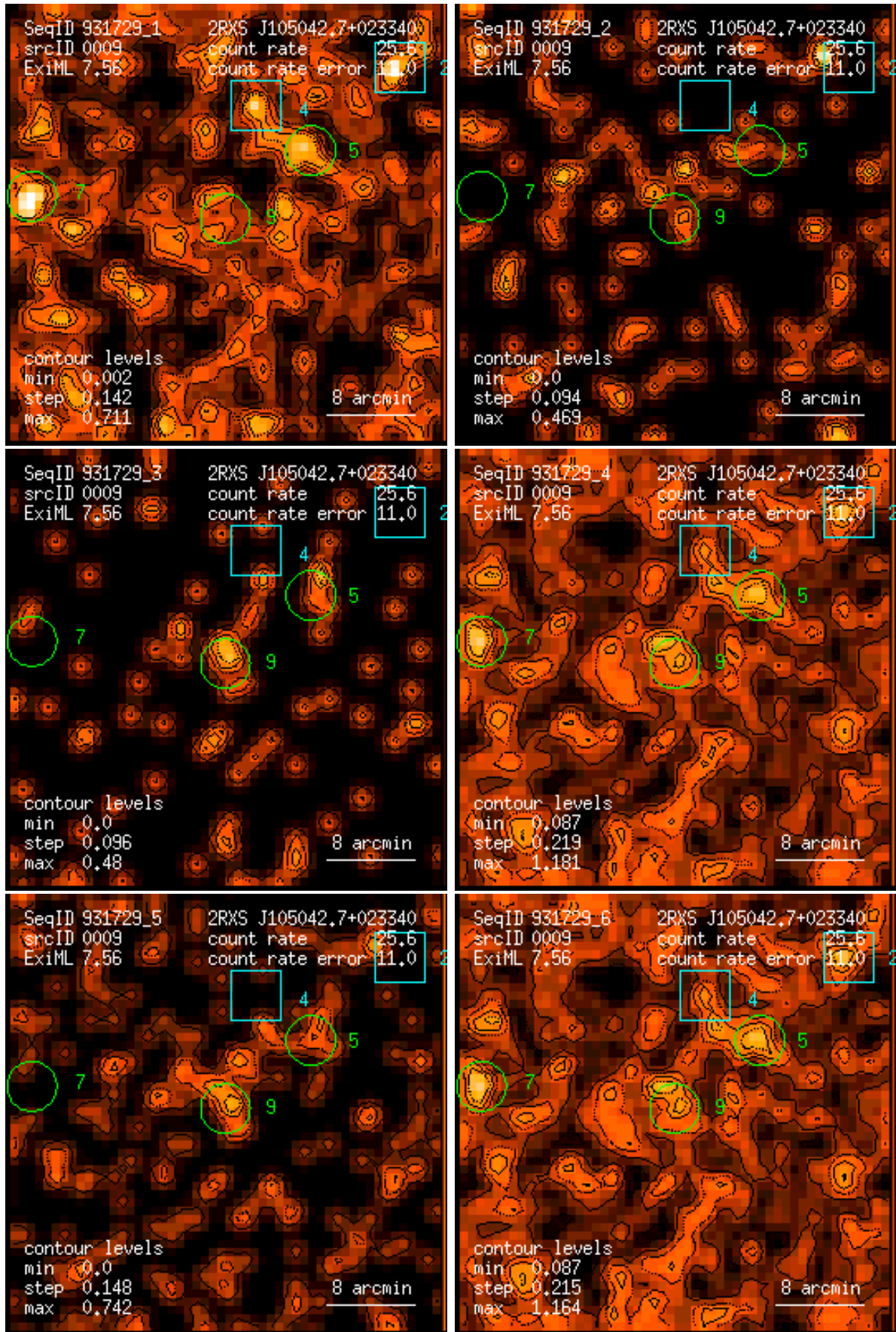
Figure 9: RASS 931729: detection 0009: band rate images, Gaussian filter: (1) PSPC channels 11 – 41, (2) 52 – 90, (3) 91 – 201, (4) 11 – 235, (5) 52 – 201, (6) 11 – 201. Broad band rates in counts/ks. Band rate contour levels in counts/ks/arcmin 2 .
