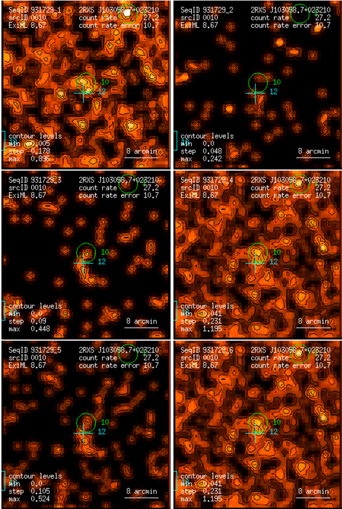
Figure 10: RASS 931729: detection 0010: band rate images, Gaussian filter: (1) PSPC channels 11 – 41, (2) 52 – 90, (3) 91 – 201, (4) 11 – 235, (5) 52 – 201, (6) 11 – 201. Broad band rates in counts/ks. Band rate contour levels in counts/ks/arcmin 2 .
