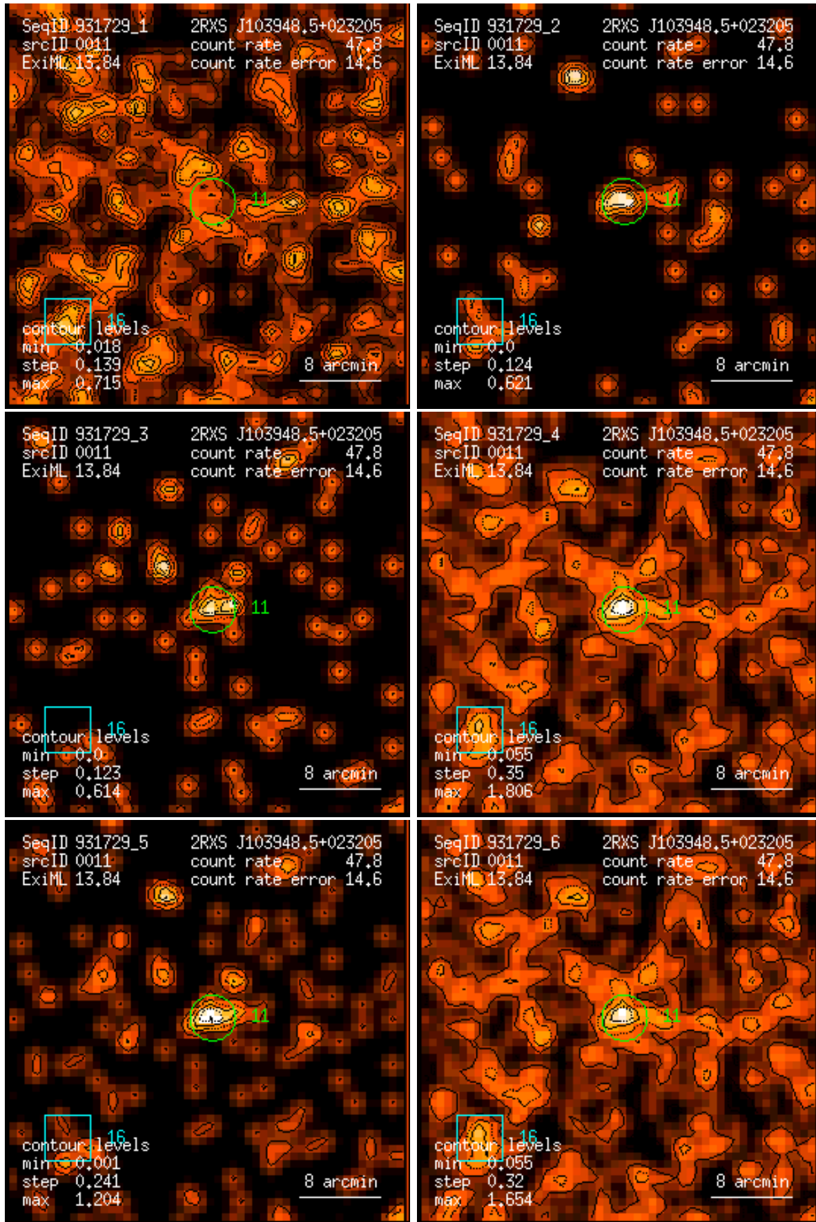
Figure 11: RASS 931729: detection 0011: band rate images, Gaussian filter: (1) PSPC channels 11 – 41, (2) 52 – 90, (3) 91 – 201, (4) 11 – 235, (5) 52 – 201, (6) 11 – 201. Broad band rates in counts/ks. Band rate contour levels in counts/ks/arcmin 2 .
