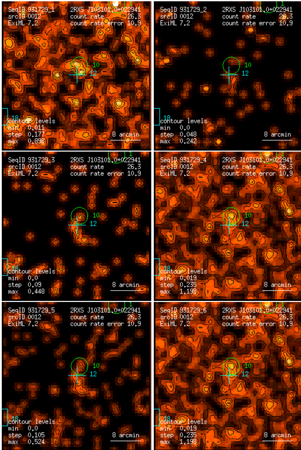
Figure 12: RASS 931729: detection 0012: band rate images, Gaussian filter: (1) PSPC channels 11 – 41, (2) 52 – 90, (3) 91 – 201, (4) 11 – 235, (5) 52 – 201, (6) 11 – 201. Broad band rates in counts/ks. Band rate contour levels in counts/ks/arcmin 2 .
