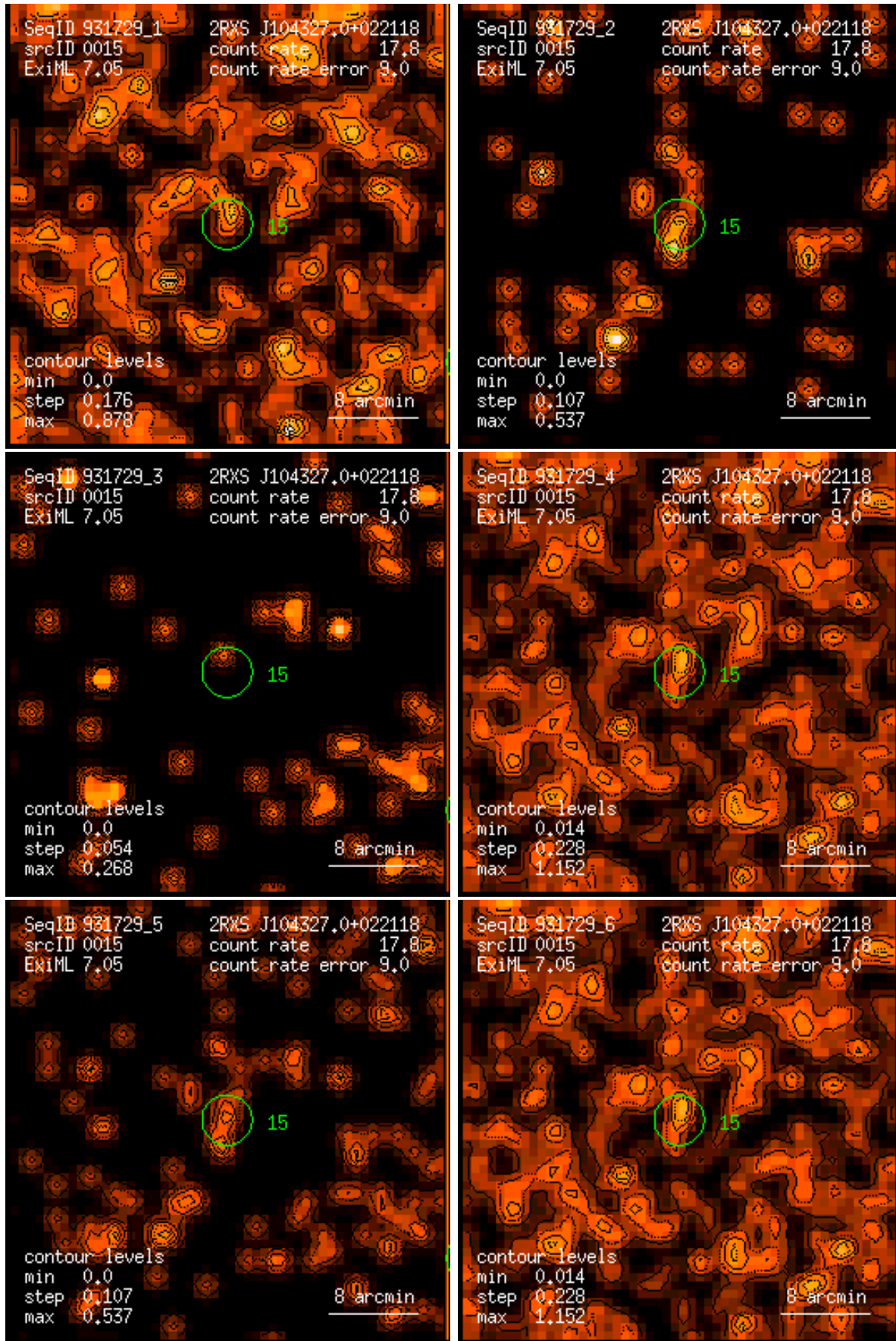
Figure 15: RASS 931729: detection 0015: band rate images, Gaussian filter: (1) PSPC channels 11 – 41, (2) 52 – 90, (3) 91 – 201, (4) 11 – 235, (5) 52 – 201, (6) 11 – 201. Broad band rates in counts/ks. Band rate contour levels in counts/ks/arcmin 2 .
