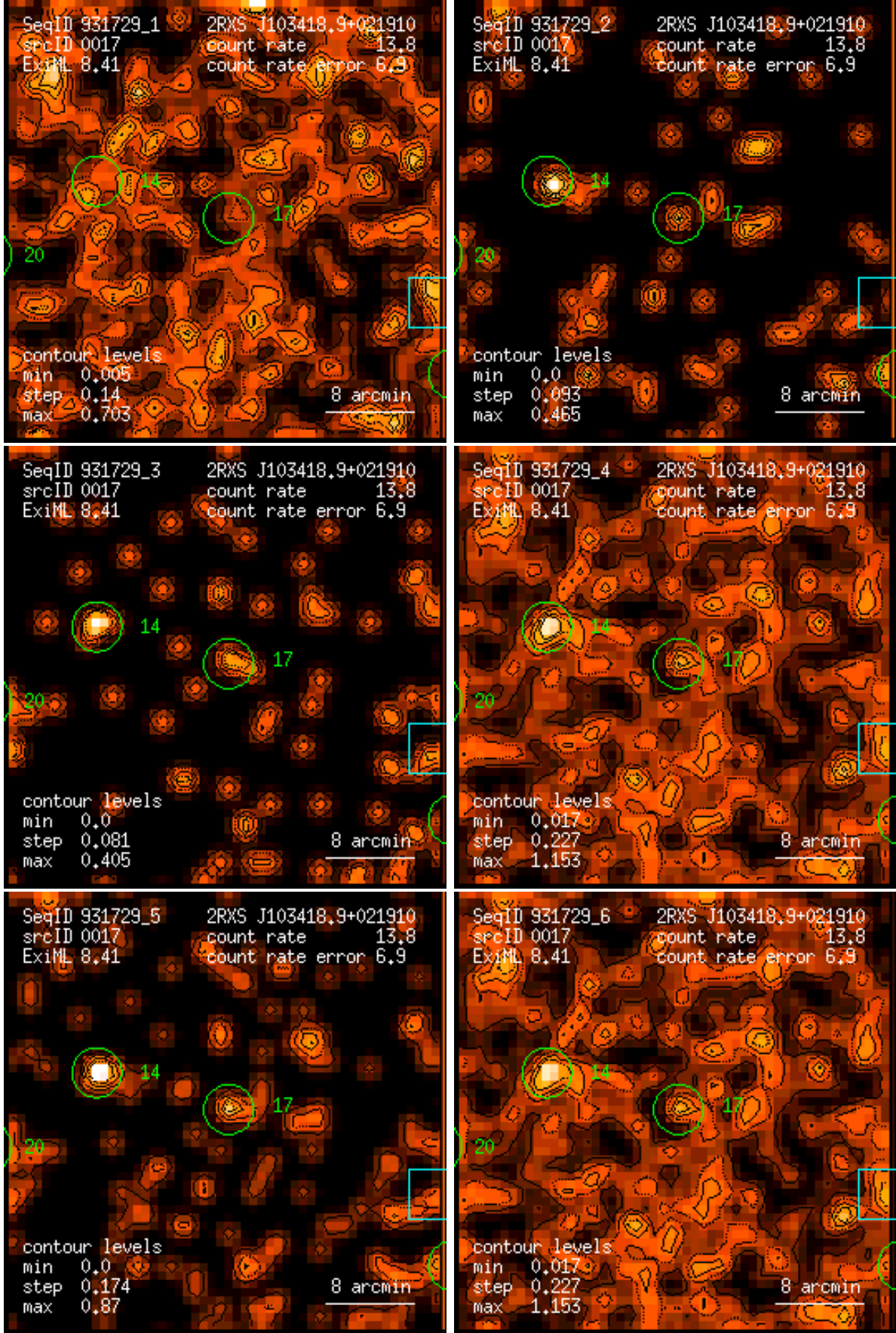
Figure 17: RASS 931729: detection 0017: band rate images, Gaussian filter: (1) PSPC channels 11 – 41, (2) 52 – 90, (3) 91 – 201, (4) 11 – 235, (5) 52 – 201, (6) 11 – 201. Broad band rates in counts/ks. Band rate contour levels in counts/ks/arcmin 2 .
