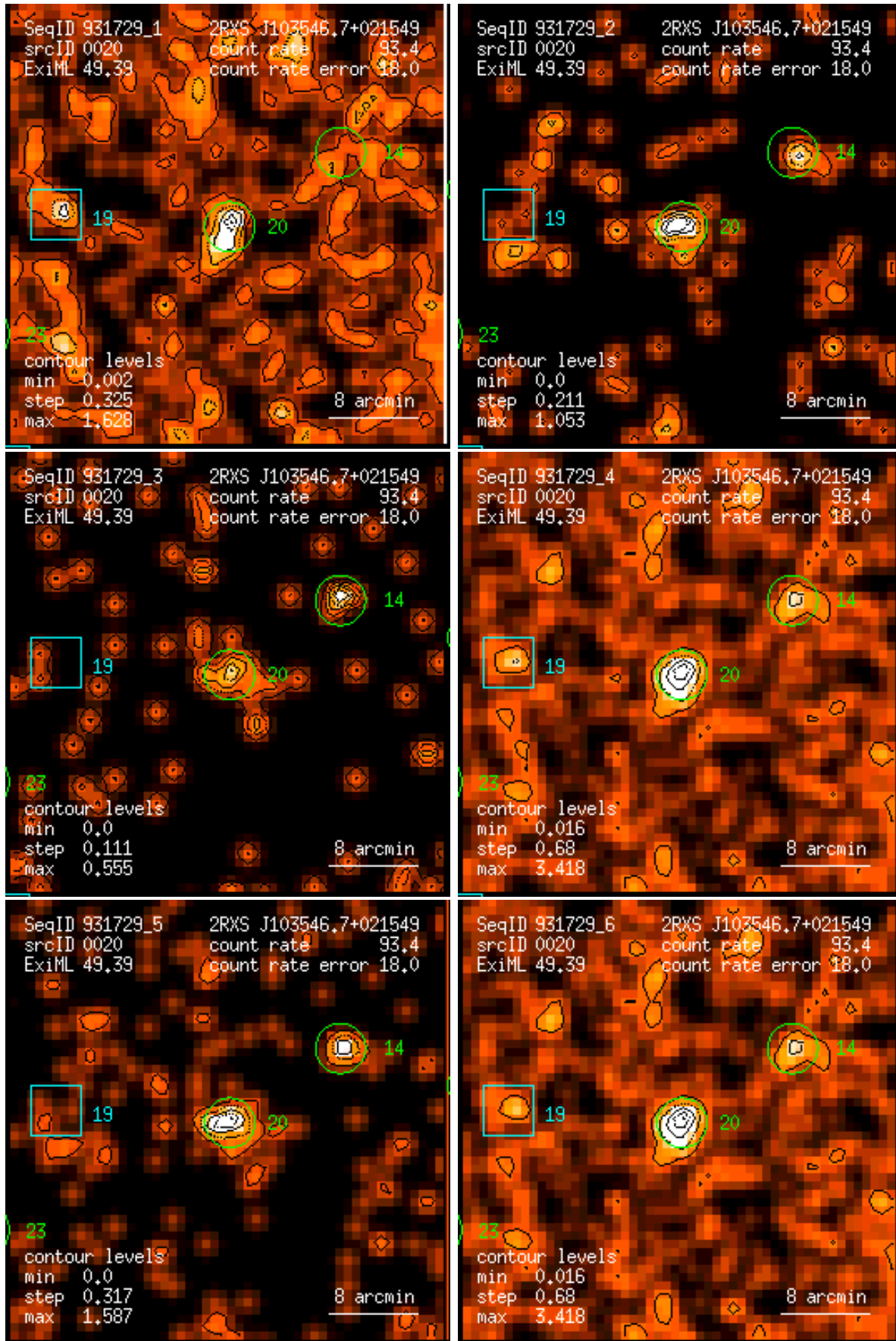
Figure 20: RASS 931729: detection 0020: band rate images, Gaussian filter: (1) PSPC channels 11 – 41, (2) 52 – 90, (3) 91 – 201, (4) 11 – 235, (5) 52 – 201, (6) 11 – 201. Broad band rates in counts/ks. Band rate contour levels in counts/ks/arcmin 2 .
