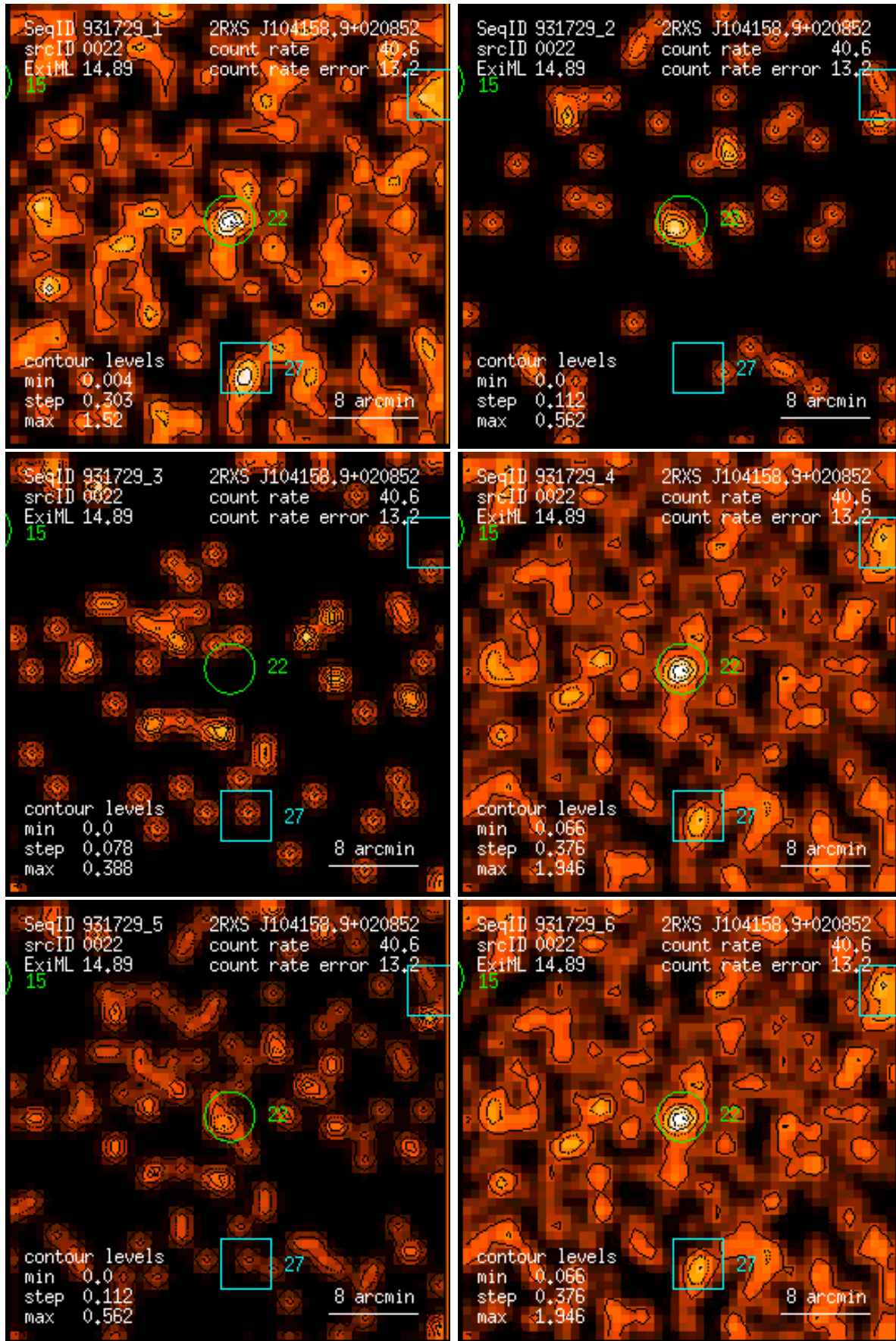
Figure 22: RASS 931729: detection 0022: band rate images, Gaussian filter: (1) PSPC channels 11 – 41, (2) 52 – 90, (3) 91 – 201, (4) 11 – 235, (5) 52 – 201, (6) 11 – 201. Broad band rates in counts/ks. Band rate contour levels in counts/ks/arcmin 2 .
