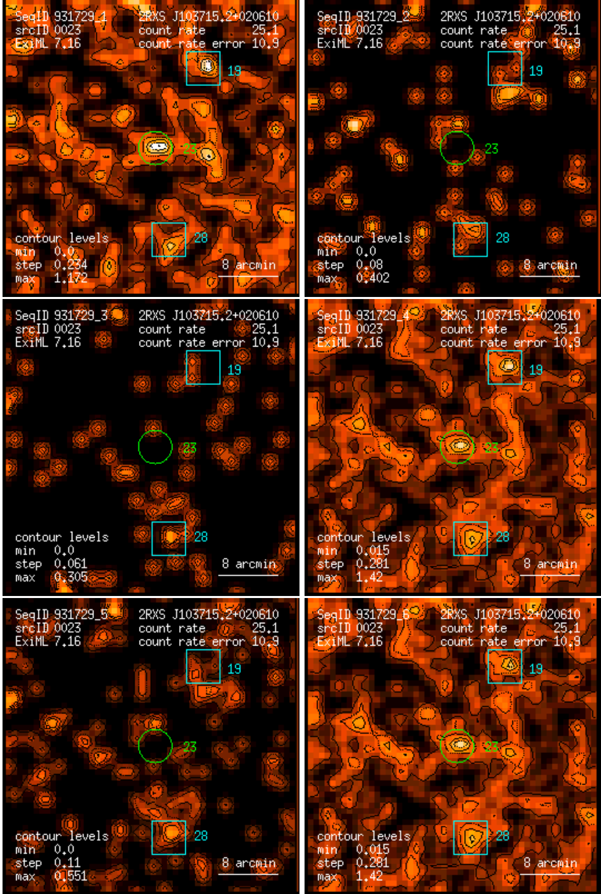
Figure 23: RASS 931729: detection 0023: band rate images, Gaussian filter: (1) PSPC channels 11 – 41, (2) 52 – 90, (3) 91 – 201, (4) 11 – 235, (5) 52 – 201, (6) 11 – 201. Broad band rates in counts/ks. Band rate contour levels in counts/ks/arcmin 2 .
