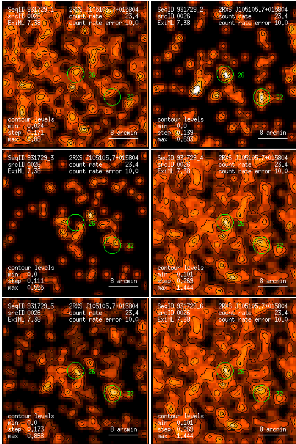
Figure 26: RASS 931729: detection 0026: band rate images, Gaussian filter: (1) PSPC channels 11 – 41, (2) 52 – 90, (3) 91 – 201, (4) 11 – 235, (5) 52 – 201, (6) 11 – 201. Broad band rates in counts/ks. Band rate contour levels in counts/ks/arcmin 2 .
