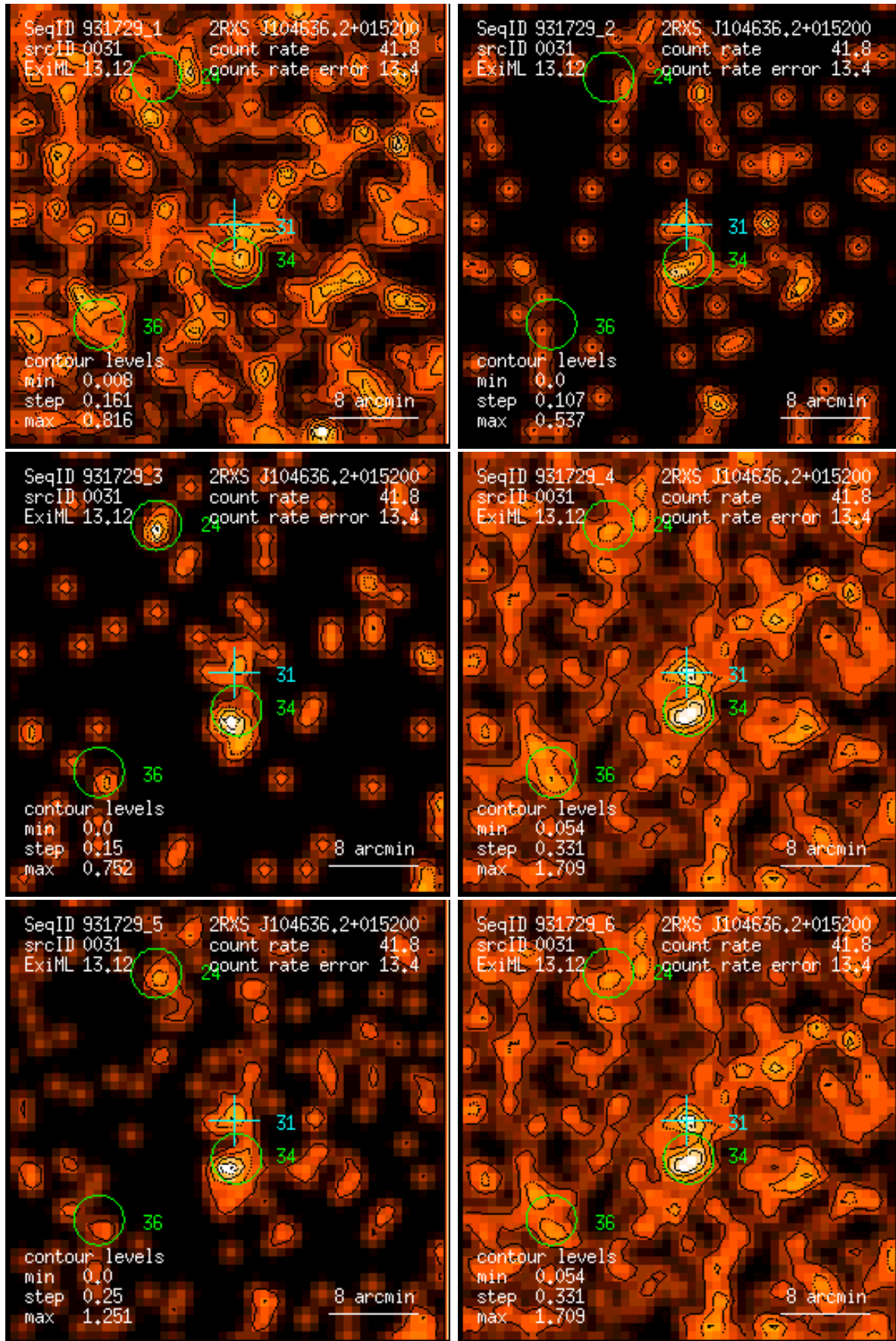
Figure 31: RASS 931729: detection 0031: band rate images, Gaussian filter: (1) PSPC channels 11 – 41, (2) 52 – 90, (3) 91 – 201, (4) 11 – 235, (5) 52 – 201, (6) 11 – 201. Broad band rates in counts/ks. Band rate contour levels in counts/ks/arcmin 2 .
