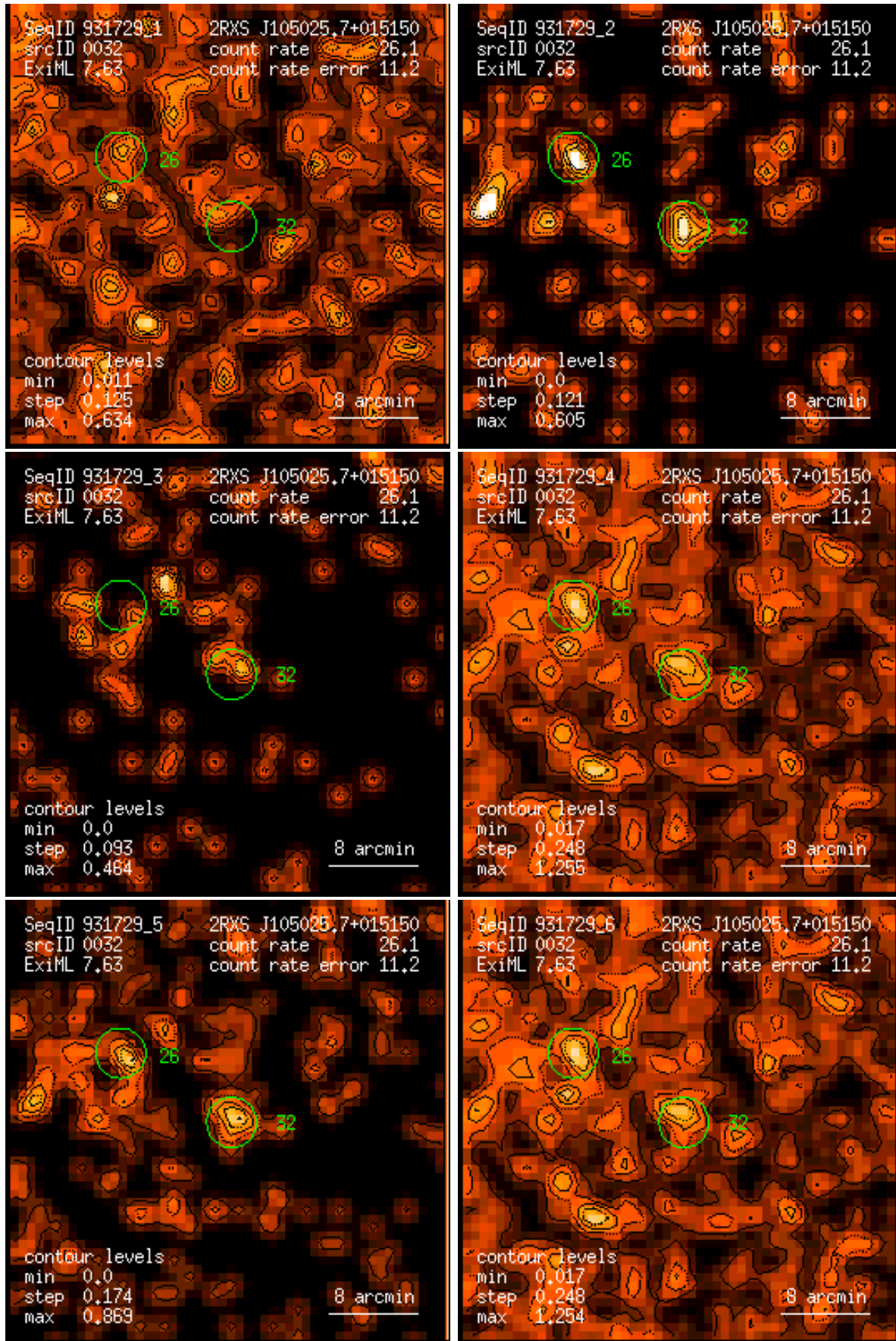
Figure 32: RASS 931729: detection 0032: band rate images, Gaussian filter: (1) PSPC channels 11 – 41, (2) 52 – 90, (3) 91 – 201, (4) 11 – 235, (5) 52 – 201, (6) 11 – 201. Broad band rates in counts/ks. Band rate contour levels in counts/ks/arcmin 2 .
