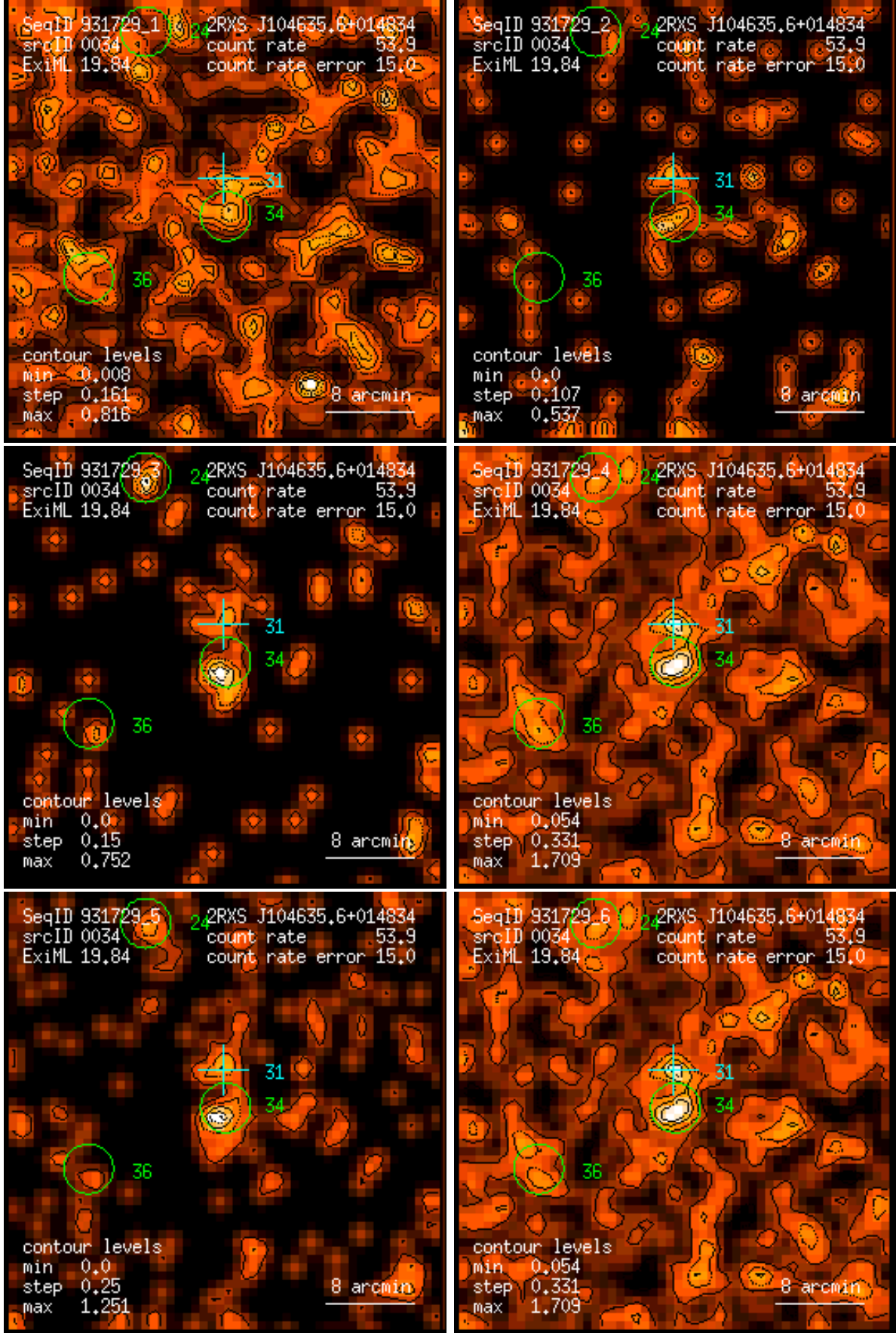
Figure 34: RASS 931729: detection 0034: band rate images, Gaussian filter: (1) PSPC channels 11 – 41, (2) 52 – 90, (3) 91 – 201, (4) 11 – 235, (5) 52 – 201, (6) 11 – 201. Broad band rates in counts/ks. Band rate contour levels in counts/ks/arcmin 2 .
