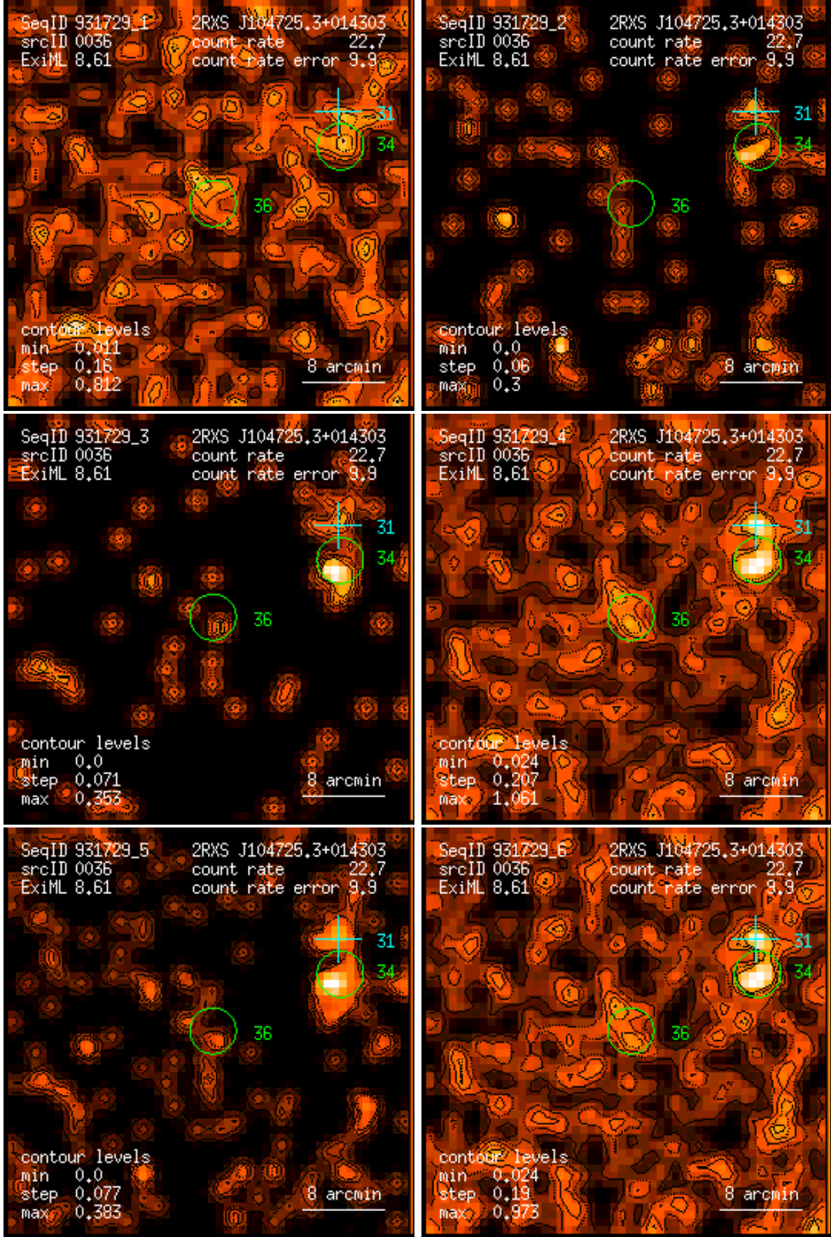
Figure 36: RASS 931729: detection 0036: band rate images, Gaussian filter: (1) PSPC channels 11 – 41, (2) 52 – 90, (3) 91 – 201, (4) 11 – 235, (5) 52 – 201, (6) 11 – 201. Broad band rates in counts/ks. Band rate contour levels in counts/ks/arcmin 2 .
