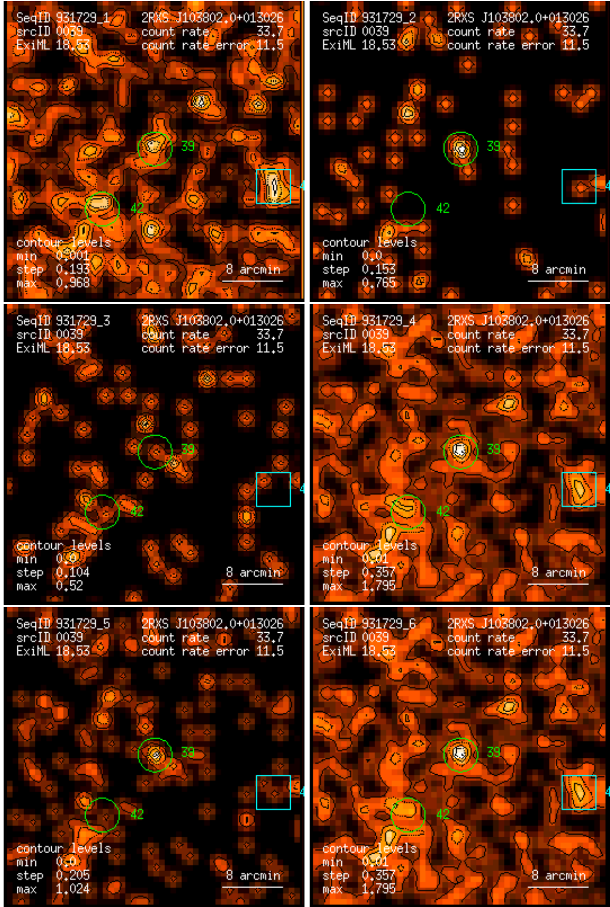
Figure 39: RASS 931729: detection 0039: band rate images, Gaussian filter: (1) PSPC channels 11 – 41, (2) 52 – 90, (3) 91 – 201, (4) 11 – 235, (5) 52 – 201, (6) 11 – 201. Broad band rates in counts/ks. Band rate contour levels in counts/ks/arcmin 2 .
