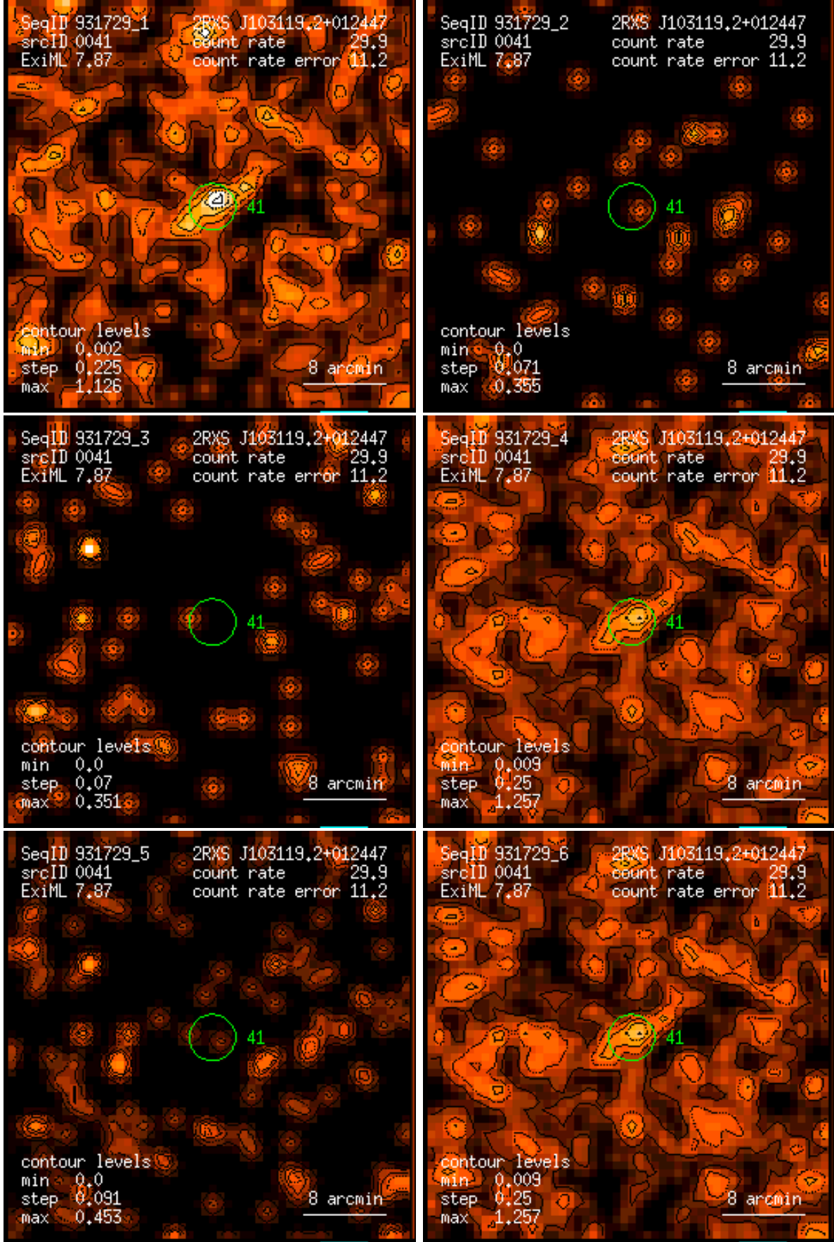
Figure 41: RASS 931729: detection 0041: band rate images, Gaussian filter: (1) PSPC channels 11 – 41, (2) 52 – 90, (3) 91 – 201, (4) 11 – 235, (5) 52 – 201, (6) 11 – 201. Broad band rates in counts/ks. Band rate contour levels in counts/ks/arcmin 2 .
