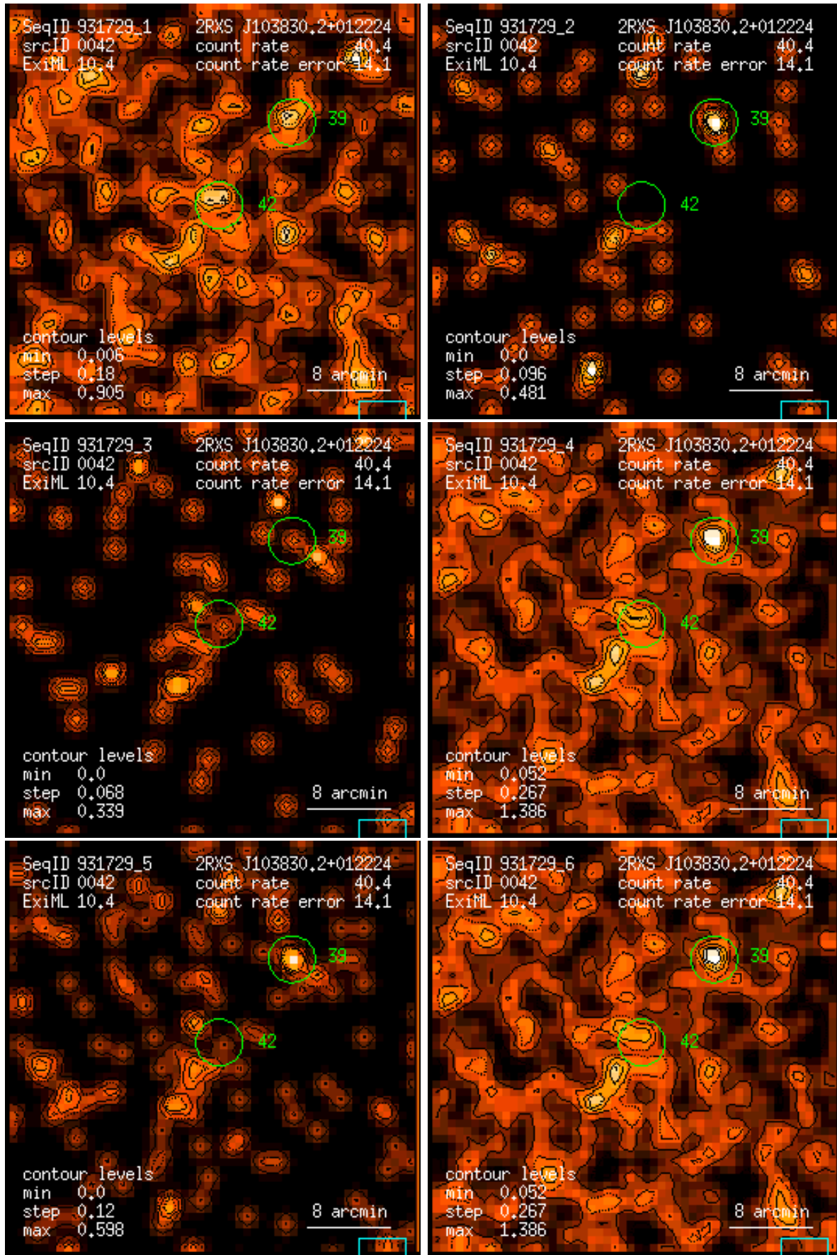
Figure 42: RASS 931729: detection 0042: band rate images, Gaussian filter: (1) PSPC channels 11 – 41, (2) 52 – 90, (3) 91 – 201, (4) 11 – 235, (5) 52 – 201, (6) 11 – 201. Broad band rates in counts/ks. Band rate contour levels in counts/ks/arcmin 2 .
