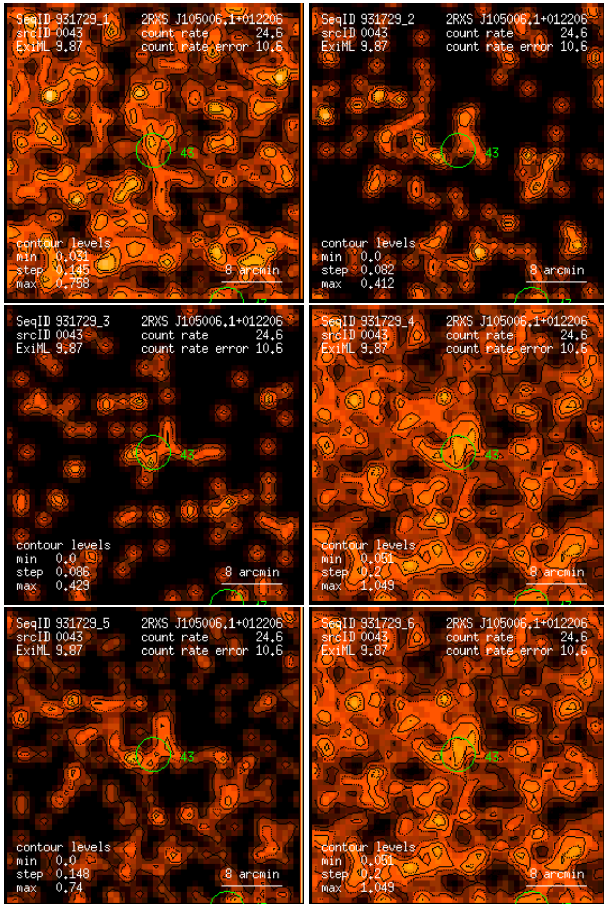
Figure 43: RASS 931729: detection 0043: band rate images, Gaussian filter: (1) PSPC channels 11 – 41, (2) 52 – 90, (3) 91 – 201, (4) 11 – 235, (5) 52 – 201, (6) 11 – 201. Broad band rates in counts/ks. Band rate contour levels in counts/ks/arcmin 2 .
