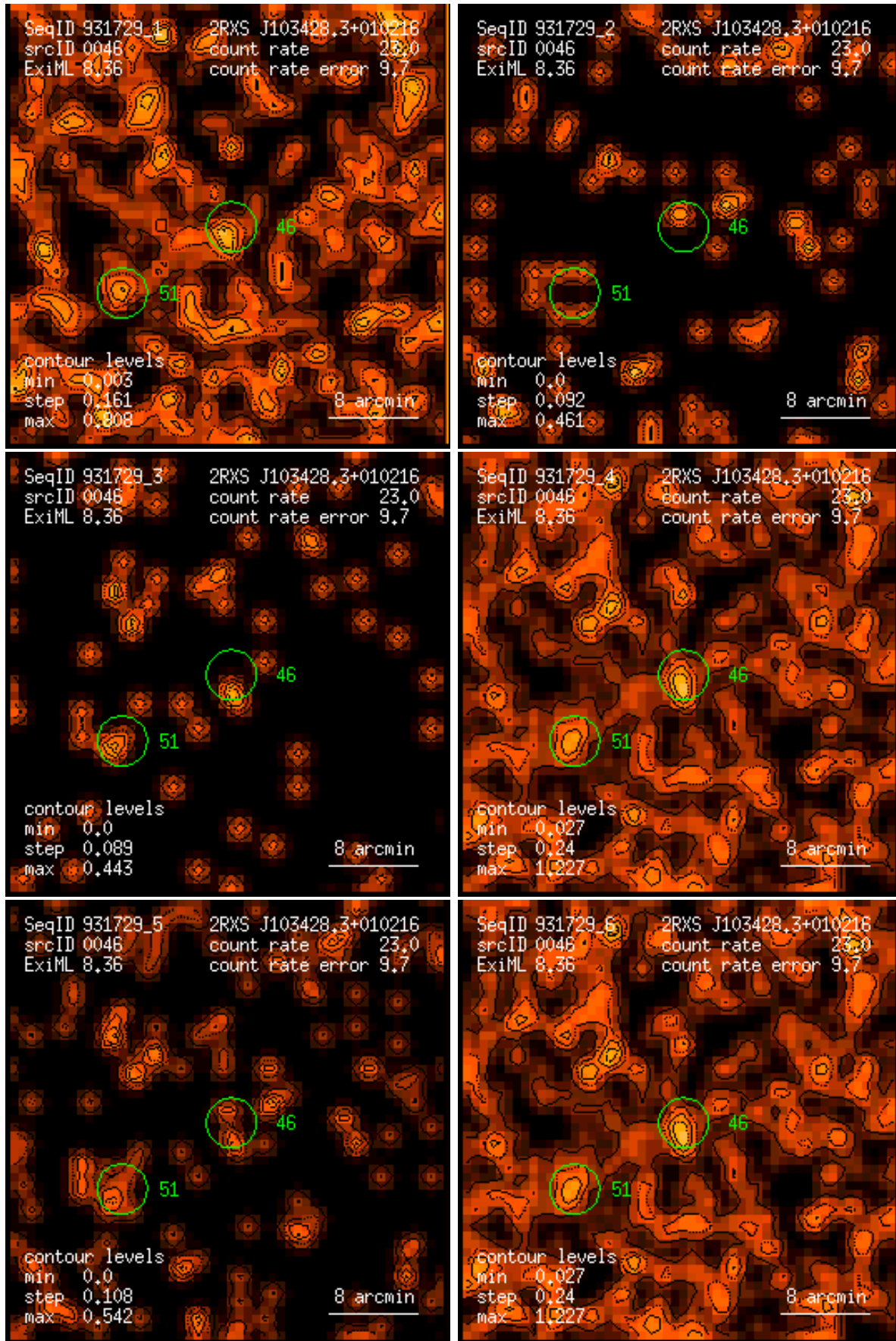
Figure 46: RASS 931729: detection 0046: band rate images, Gaussian filter: (1) PSPC channels 11 – 41, (2) 52 – 90, (3) 91 – 201, (4) 11 – 235, (5) 52 – 201, (6) 11 – 201. Broad band rates in counts/ks. Band rate contour levels in counts/ks/arcmin 2 .
