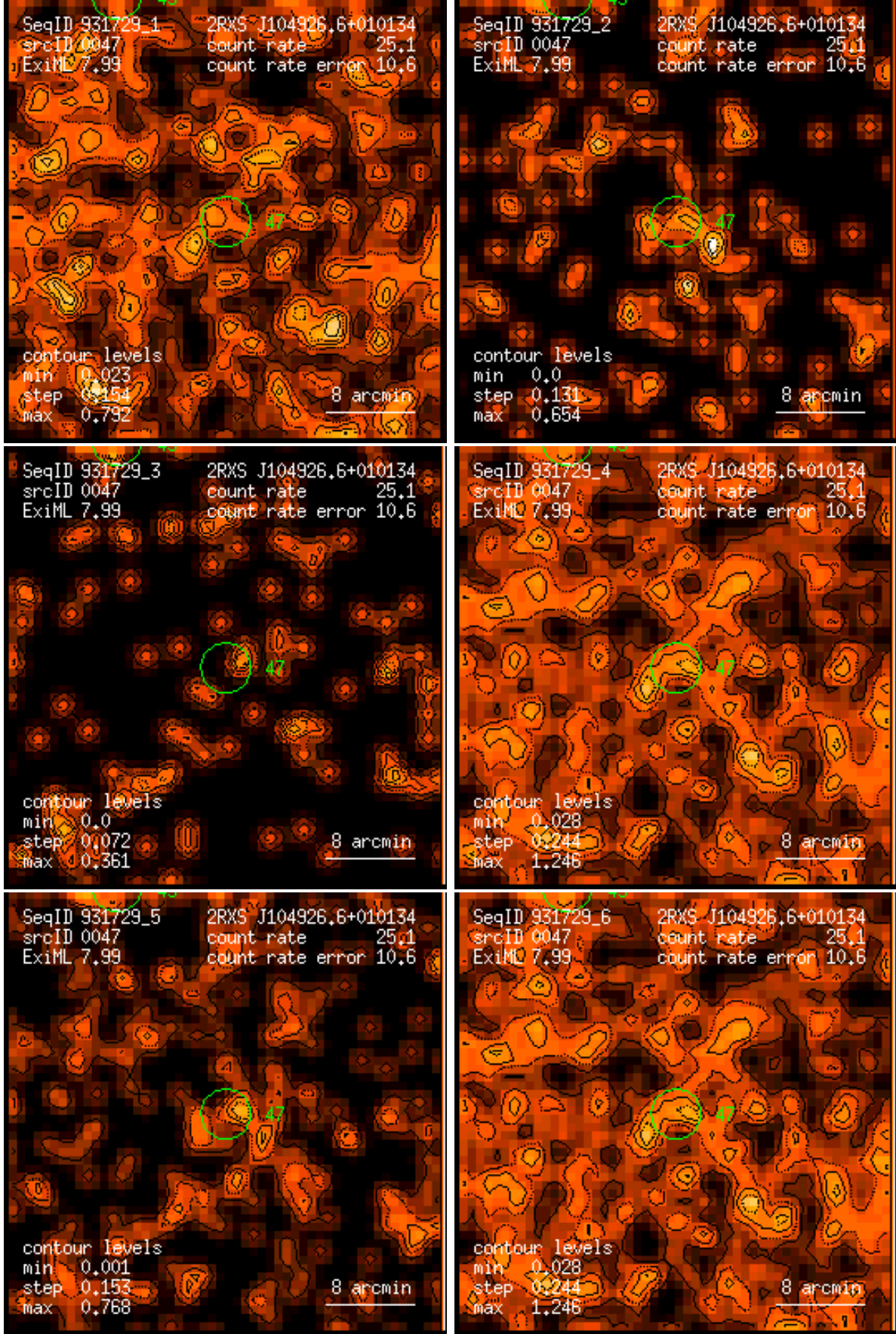
Figure 47: RASS 931729: detection 0047: band rate images, Gaussian filter: (1) PSPC channels 11 – 41, (2) 52 – 90, (3) 91 – 201, (4) 11 – 235, (5) 52 – 201, (6) 11 – 201. Broad band rates in counts/ks. Band rate contour levels in counts/ks/arcmin 2 .
