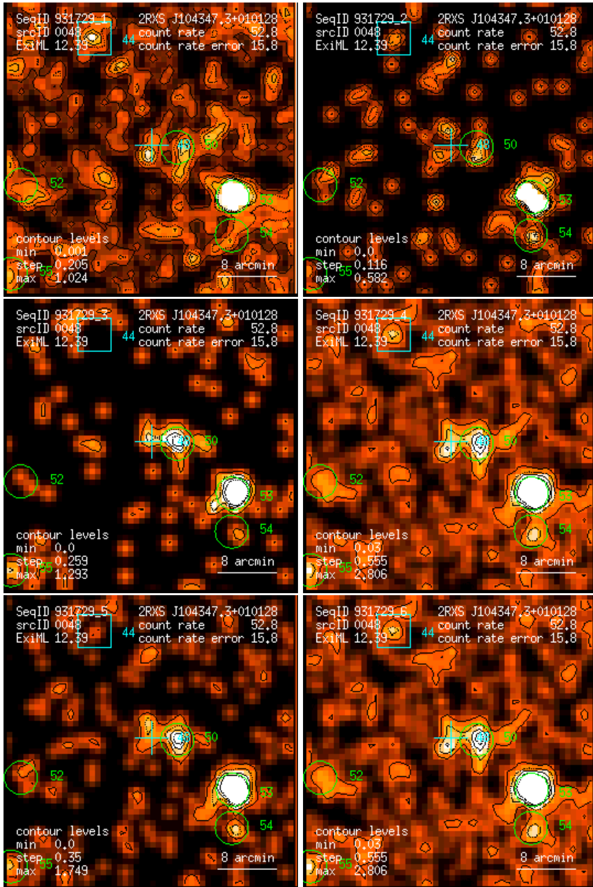
Figure 48: RASS 931729: detection 0048: band rate images, Gaussian filter: (1) PSPC channels 11 – 41, (2) 52 – 90, (3) 91 – 201, (4) 11 – 235, (5) 52 – 201, (6) 11 – 201. Broad band rates in counts/ks. Band rate contour levels in counts/ks/arcmin 2 .
