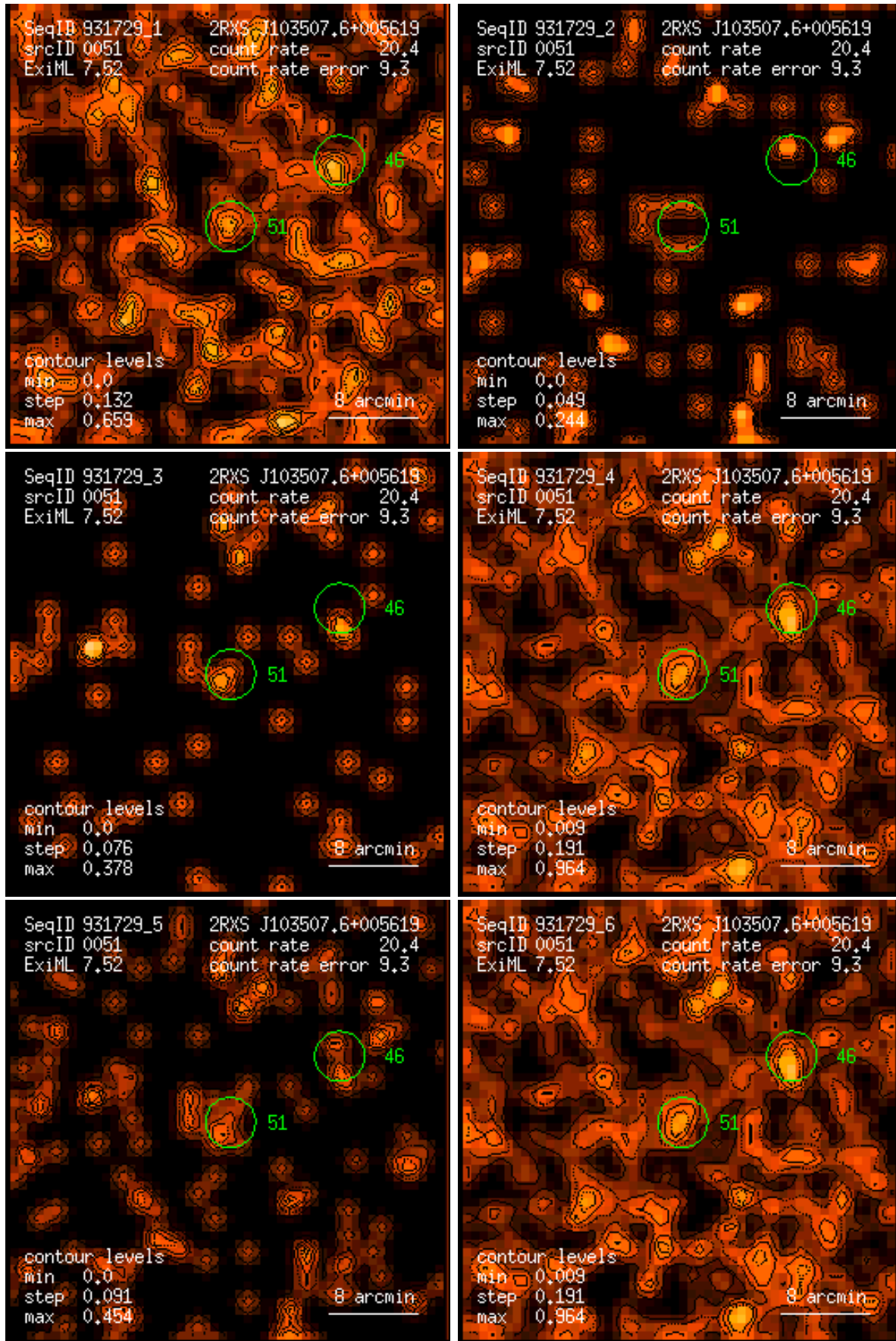
Figure 51: RASS 931729: detection 0051: band rate images, Gaussian filter: (1) PSPC channels 11 – 41, (2) 52 – 90, (3) 91 – 201, (4) 11 – 235, (5) 52 – 201, (6) 11 – 201. Broad band rates in counts/ks. Band rate contour levels in counts/ks/arcmin 2 .
