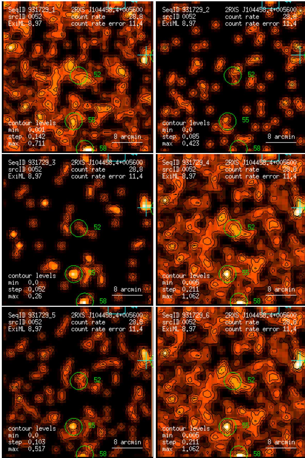
Figure 52: RASS 931729: detection 0052: band rate images, Gaussian filter: (1) PSPC channels 11 – 41, (2) 52 – 90, (3) 91 – 201, (4) 11 – 235, (5) 52 – 201, (6) 11 – 201. Broad band rates in counts/ks. Band rate contour levels in counts/ks/arcmin 2 .
