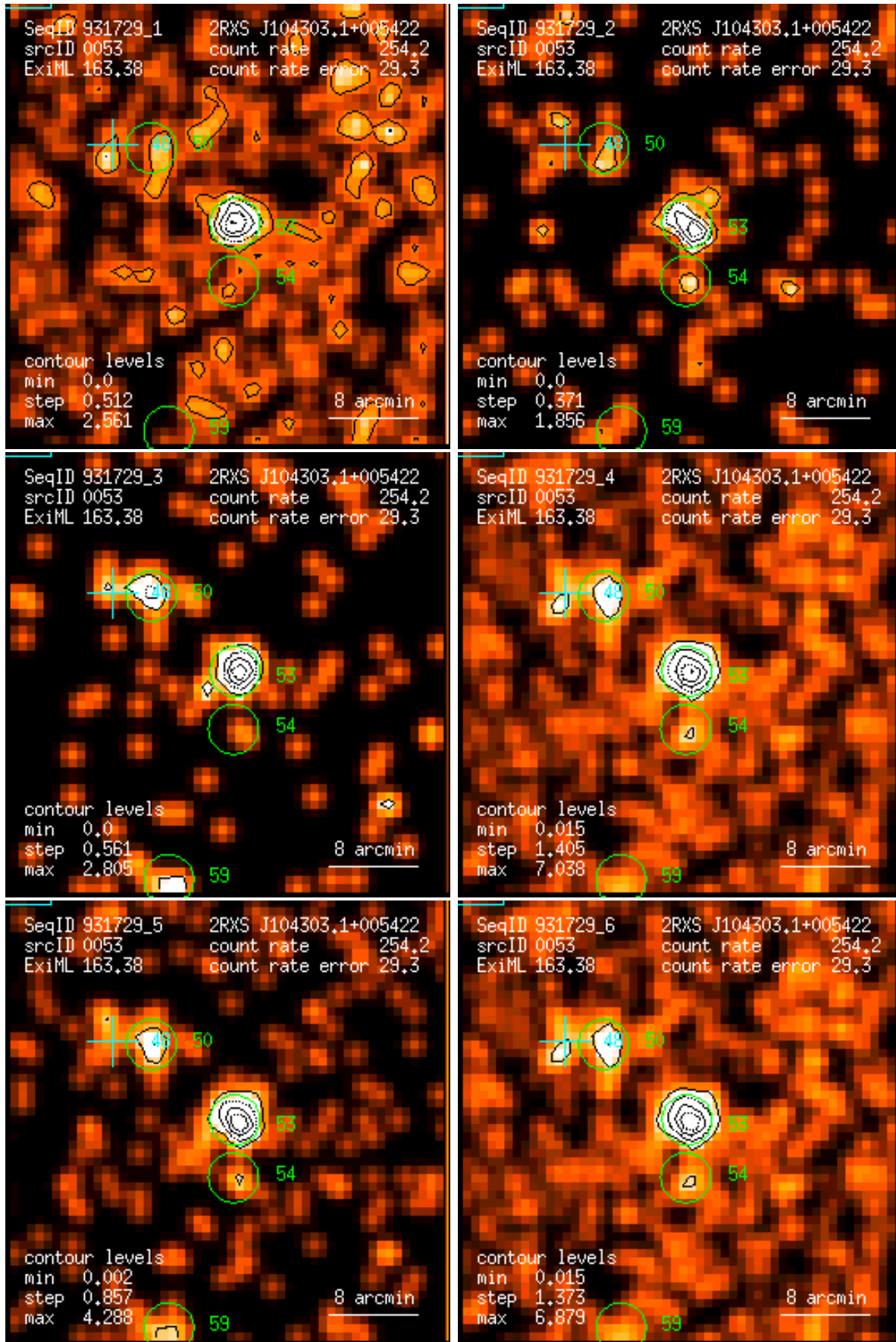
Figure 53: RASS 931729: detection 0053: band rate images, Gaussian filter: (1) PSPC channels 11 – 41, (2) 52 – 90, (3) 91 – 201, (4) 11 – 235, (5) 52 – 201, (6) 11 – 201. Broad band rates in counts/ks. Band rate contour levels in counts/ks/arcmin 2 .
