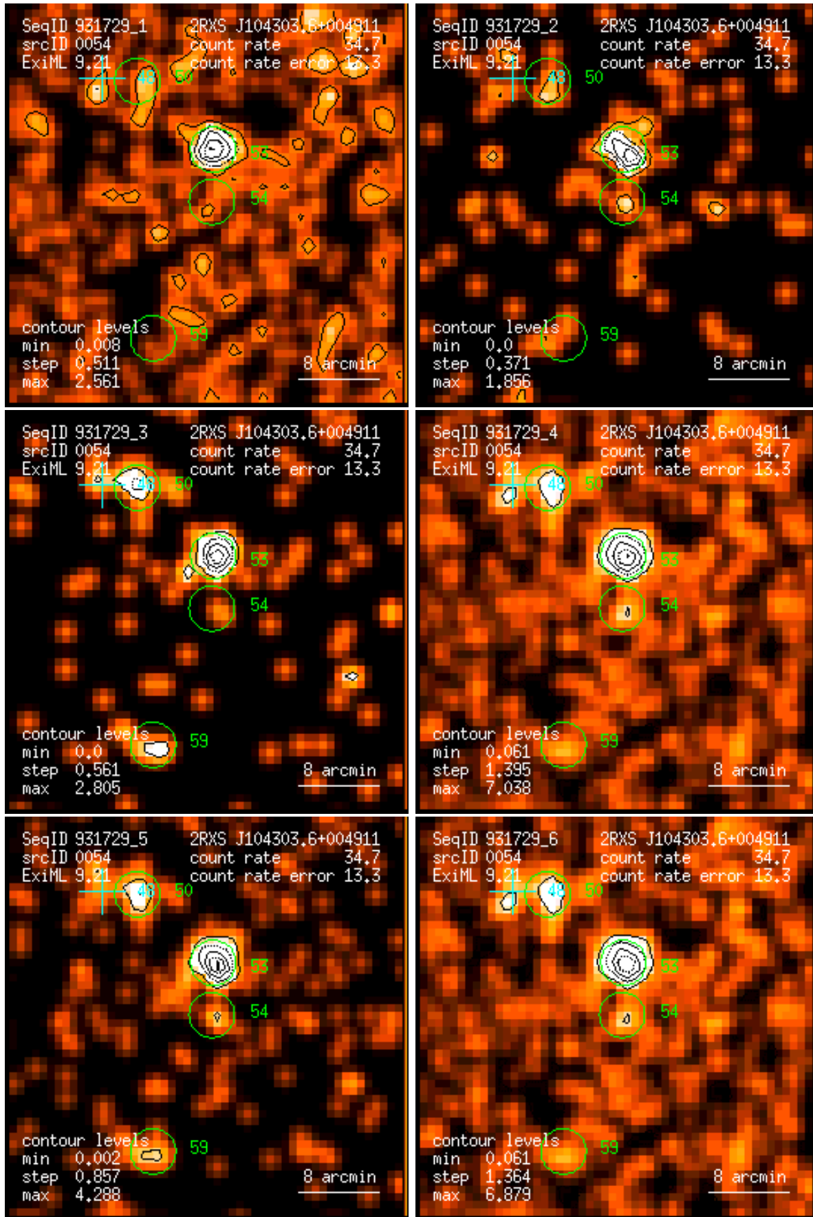
Figure 54: RASS 931729: detection 0054: band rate images, Gaussian filter: (1) PSPC channels 11 – 41, (2) 52 – 90, (3) 91 – 201, (4) 11 – 235, (5) 52 – 201, (6) 11 – 201. Broad band rates in counts/ks. Band rate contour levels in counts/ks/arcmin 2 .
