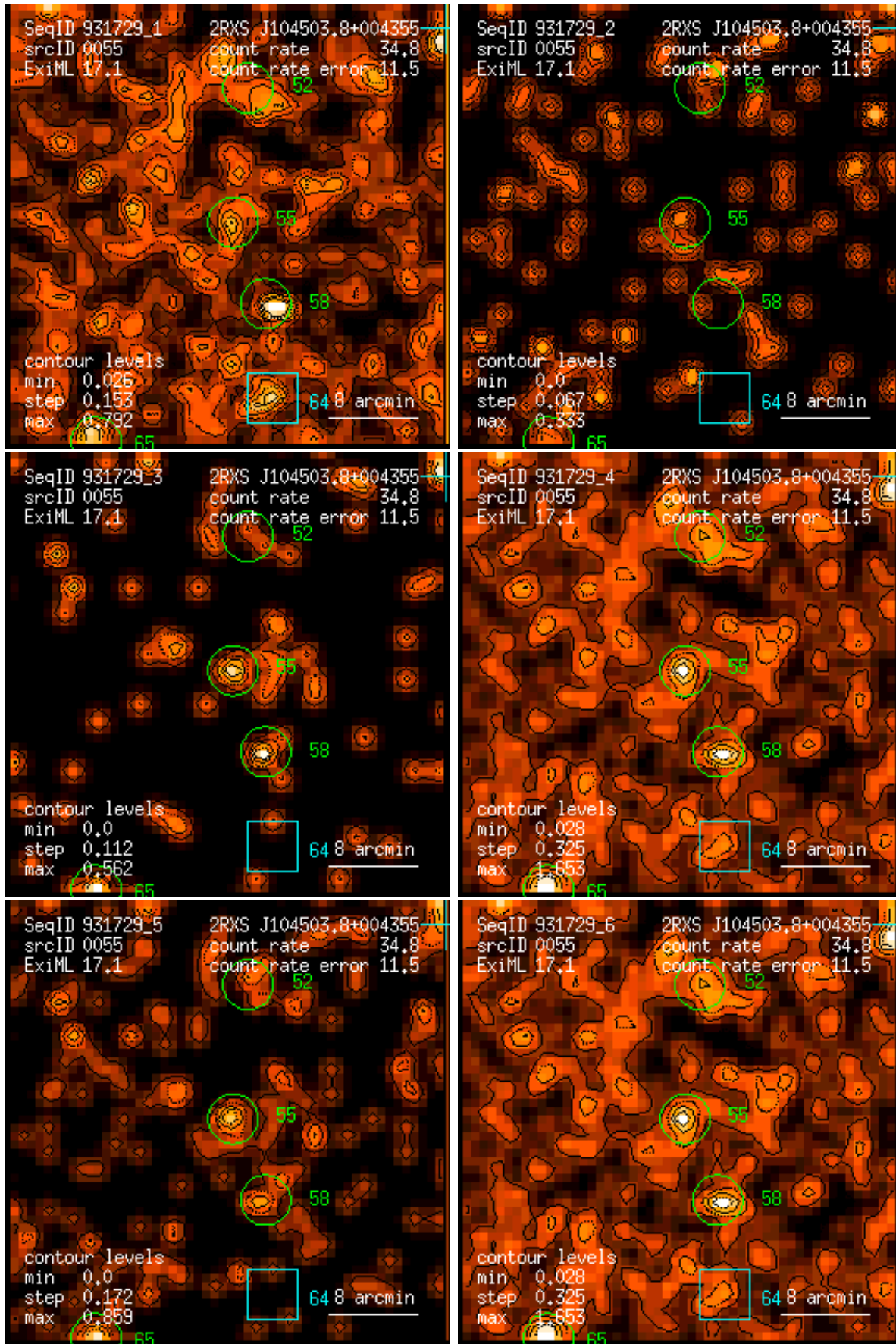
Figure 55: RASS 931729: detection 0055: band rate images, Gaussian filter: (1) PSPC channels 11 – 41, (2) 52 – 90, (3) 91 – 201, (4) 11 – 235, (5) 52 – 201, (6) 11 – 201. Broad band rates in counts/ks. Band rate contour levels in counts/ks/arcmin 2 .
