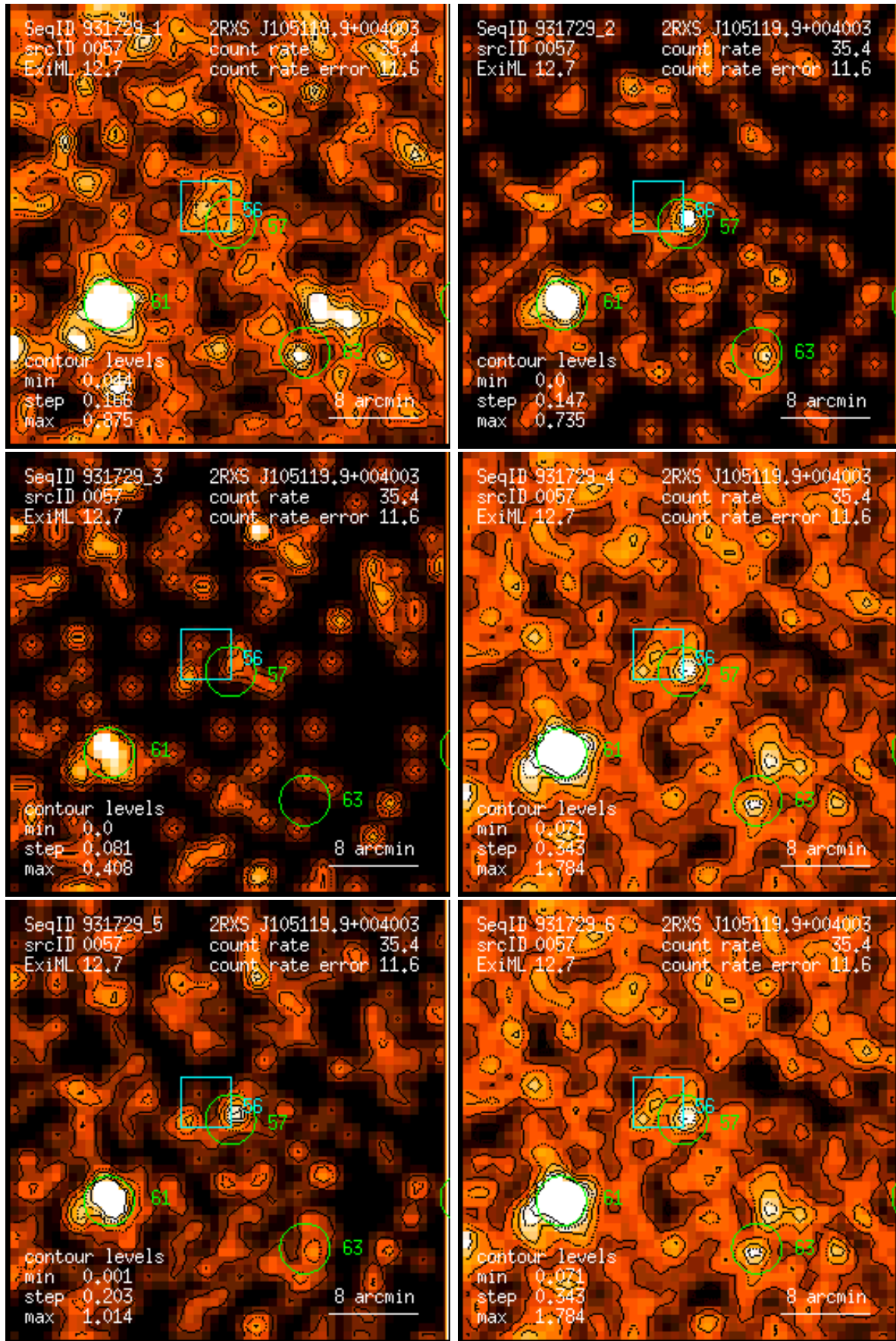
Figure 57: RASS 931729: detection 0057: band rate images, Gaussian filter: (1) PSPC channels 11 – 41, (2) 52 – 90, (3) 91 – 201, (4) 11 – 235, (5) 52 – 201, (6) 11 – 201. Broad band rates in counts/ks. Band rate contour levels in counts/ks/arcmin 2 .
