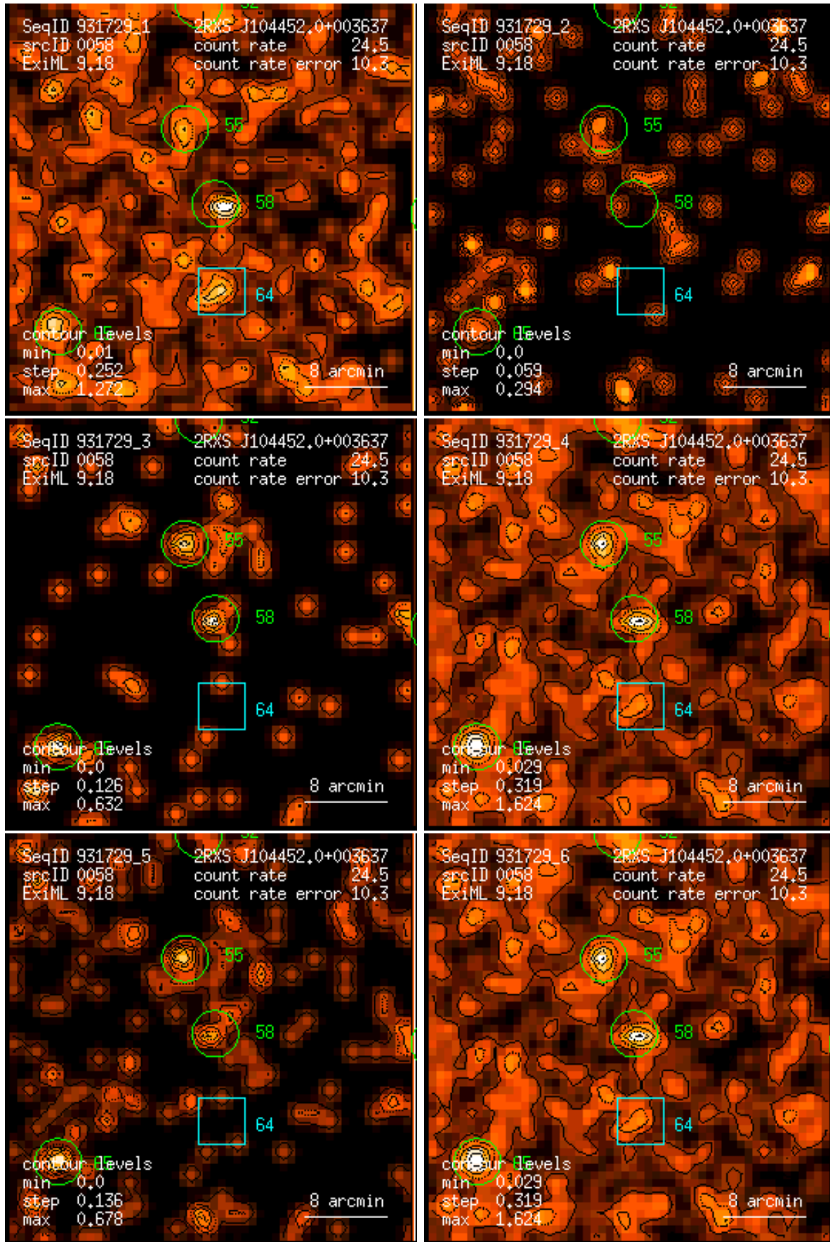
Figure 58: RASS 931729: detection 0058: band rate images, Gaussian filter: (1) PSPC channels 11 – 41, (2) 52 – 90, (3) 91 – 201, (4) 11 – 235, (5) 52 – 201, (6) 11 – 201. Broad band rates in counts/ks. Band rate contour levels in counts/ks/arcmin 2 .
