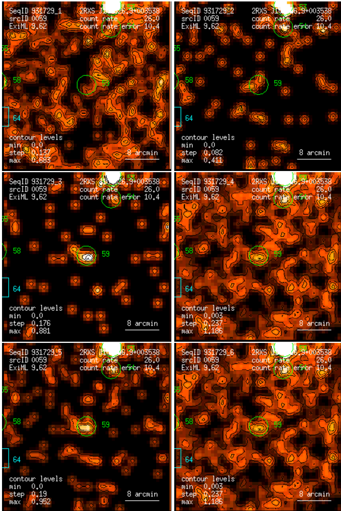
Figure 59: RASS 931729: detection 0059: band rate images, Gaussian filter: (1) PSPC channels 11 – 41, (2) 52 – 90, (3) 91 – 201, (4) 11 – 235, (5) 52 – 201, (6) 11 – 201. Broad band rates in counts/ks. Band rate contour levels in counts/ks/arcmin 2 .
