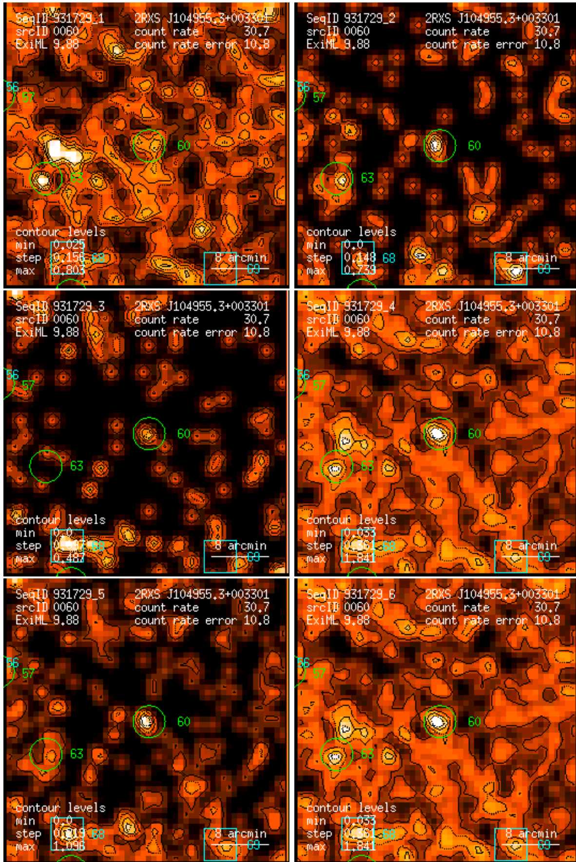
Figure 60: RASS 931729: detection 0060: band rate images, Gaussian filter: (1) PSPC channels 11 – 41, (2) 52 – 90, (3) 91 – 201, (4) 11 – 235, (5) 52 – 201, (6) 11 – 201. Broad band rates in counts/ks. Band rate contour levels in counts/ks/arcmin 2 .
