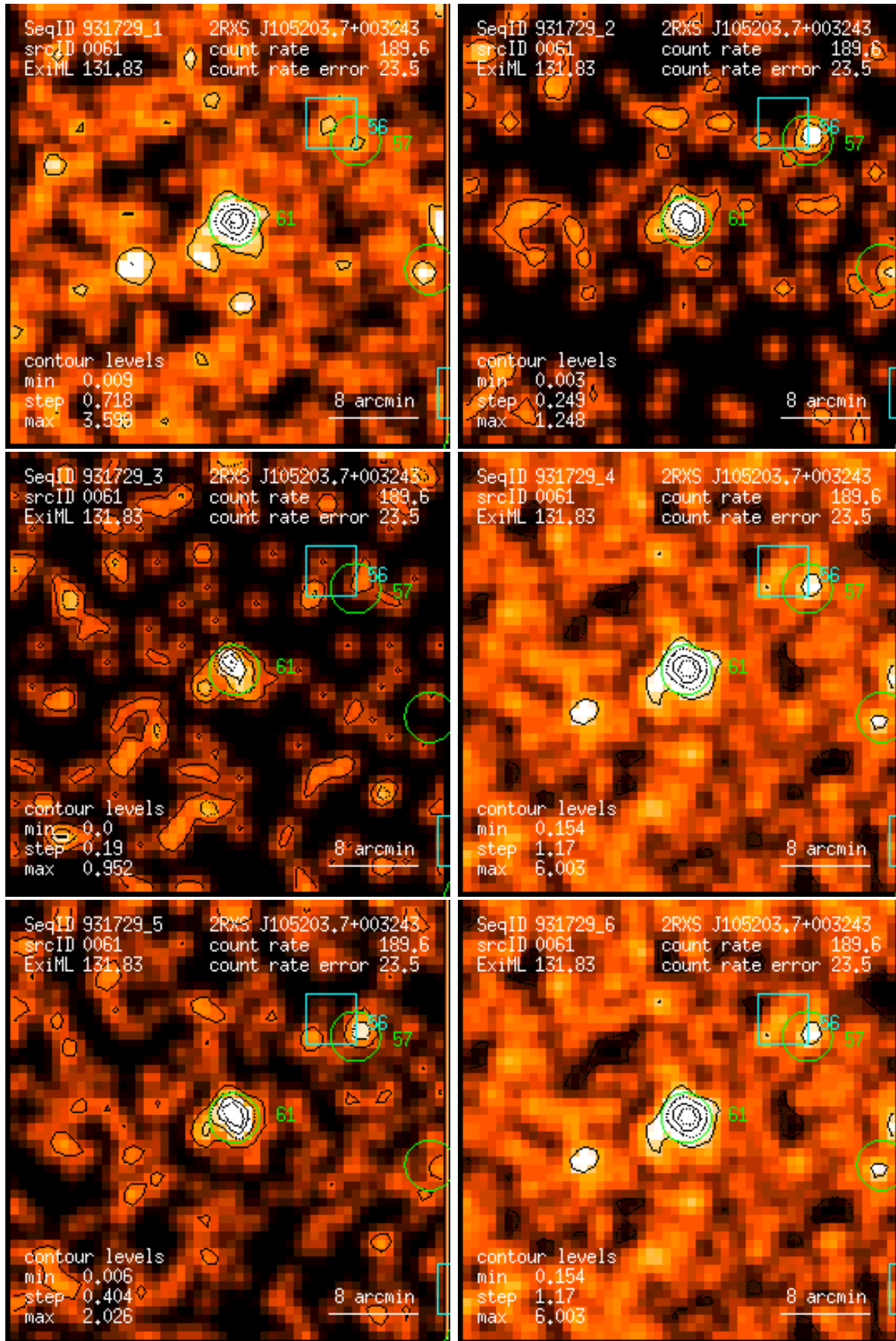
Figure 61: RASS 931729: detection 0061: band rate images, Gaussian filter: (1) PSPC channels 11 – 41, (2) 52 – 90, (3) 91 – 201, (4) 11 – 235, (5) 52 – 201, (6) 11 – 201. Broad band rates in counts/ks. Band rate contour levels in counts/ks/arcmin 2 .
