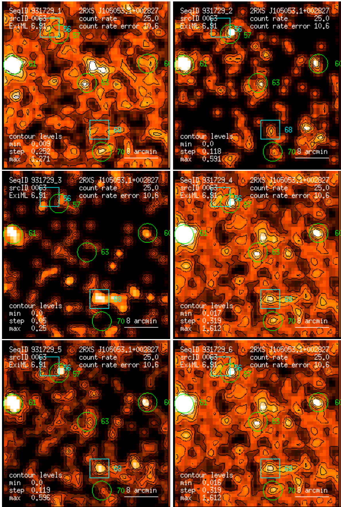
Figure 63: RASS 931729: detection 0063: band rate images, Gaussian filter: (1) PSPC channels 11 – 41, (2) 52 – 90, (3) 91 – 201, (4) 11 – 235, (5) 52 – 201, (6) 11 – 201. Broad band rates in counts/ks. Band rate contour levels in counts/ks/arcmin 2 .
