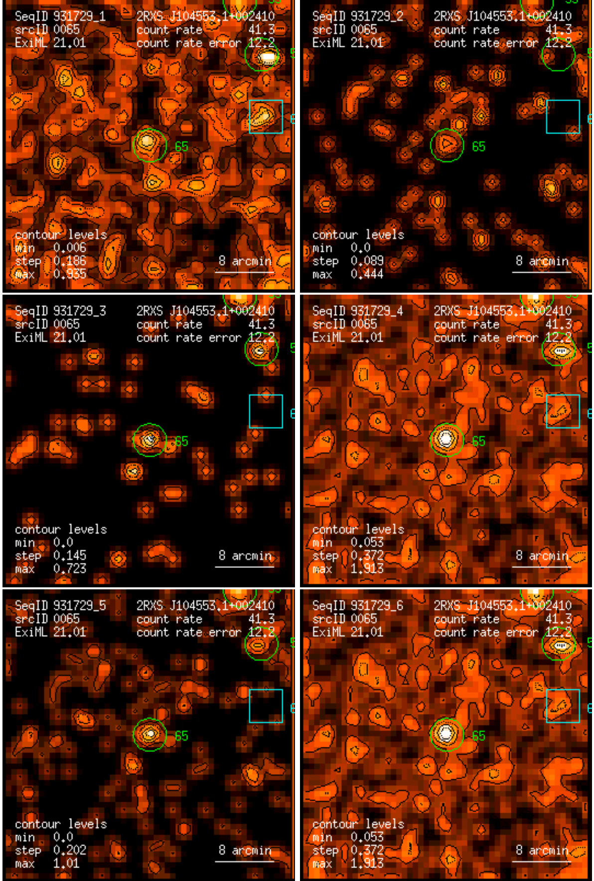
Figure 65: RASS 931729: detection 0065: band rate images, Gaussian filter: (1) PSPC channels 11 – 41, (2) 52 – 90, (3) 91 – 201, (4) 11 – 235, (5) 52 – 201, (6) 11 – 201. Broad band rates in counts/ks. Band rate contour levels in counts/ks/arcmin 2 .
