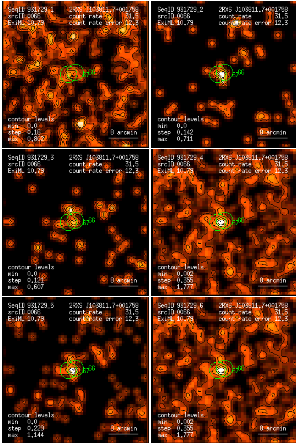
Figure 66: RASS 931729: detection 0066: band rate images, Gaussian filter: (1) PSPC channels 11 – 41, (2) 52 – 90, (3) 91 – 201, (4) 11 – 235, (5) 52 – 201, (6) 11 – 201. Broad band rates in counts/ks. Band rate contour levels in counts/ks/arcmin 2 .
