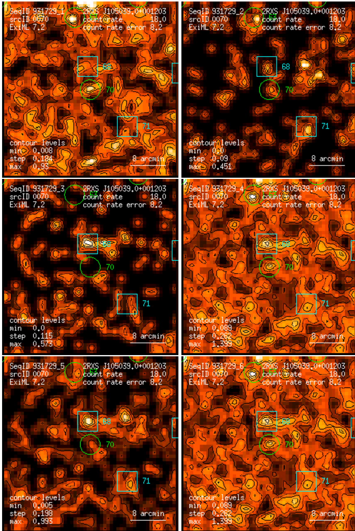
Figure 70: RASS 931729: detection 0070: band rate images, Gaussian filter: (1) PSPC channels 11 – 41, (2) 52 – 90, (3) 91 – 201, (4) 11 – 235, (5) 52 – 201, (6) 11 – 201. Broad band rates in counts/ks. Band rate contour levels in counts/ks/arcmin 2 .
