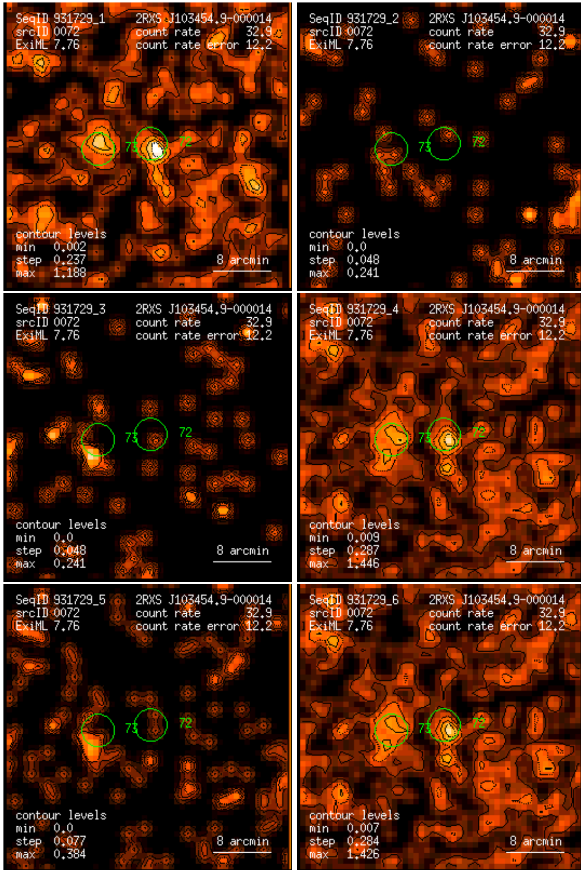
Figure 72: RASS 931729: detection 0072: band rate images, Gaussian filter: (1) PSPC channels 11 – 41, (2) 52 – 90, (3) 91 – 201, (4) 11 – 235, (5) 52 – 201, (6) 11 – 201. Broad band rates in counts/ks. Band rate contour levels in counts/ks/arcmin 2 .
