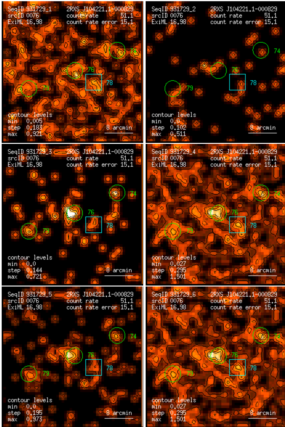
Figure 76: RASS 931729: detection 0076: band rate images, Gaussian filter: (1) PSPC channels 11 – 41, (2) 52 – 90, (3) 91 – 201, (4) 11 – 235, (5) 52 – 201, (6) 11 – 201. Broad band rates in counts/ks. Band rate contour levels in counts/ks/arcmin 2 .
