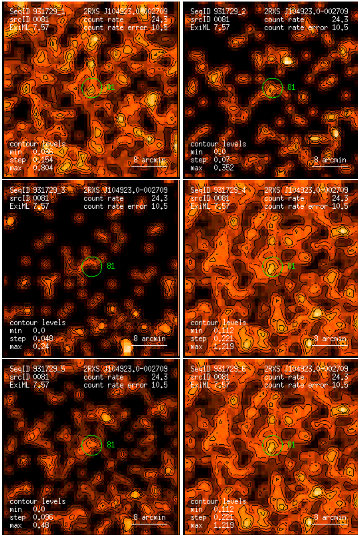
Figure 81: RASS 931729: detection 0081: band rate images, Gaussian filter: (1) PSPC channels 11 – 41, (2) 52 – 90, (3) 91 – 201, (4) 11 – 235, (5) 52 – 201, (6) 11 – 201. Broad band rates in counts/ks. Band rate contour levels in counts/ks/arcmin 2 .
