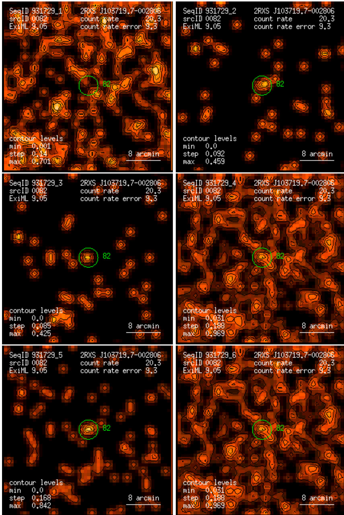
Figure 82: RASS 931729: detection 0082: band rate images, Gaussian filter: (1) PSPC channels 11 – 41, (2) 52 – 90, (3) 91 – 201, (4) 11 – 235, (5) 52 – 201, (6) 11 – 201. Broad band rates in counts/ks. Band rate contour levels in counts/ks/arcmin 2 .
