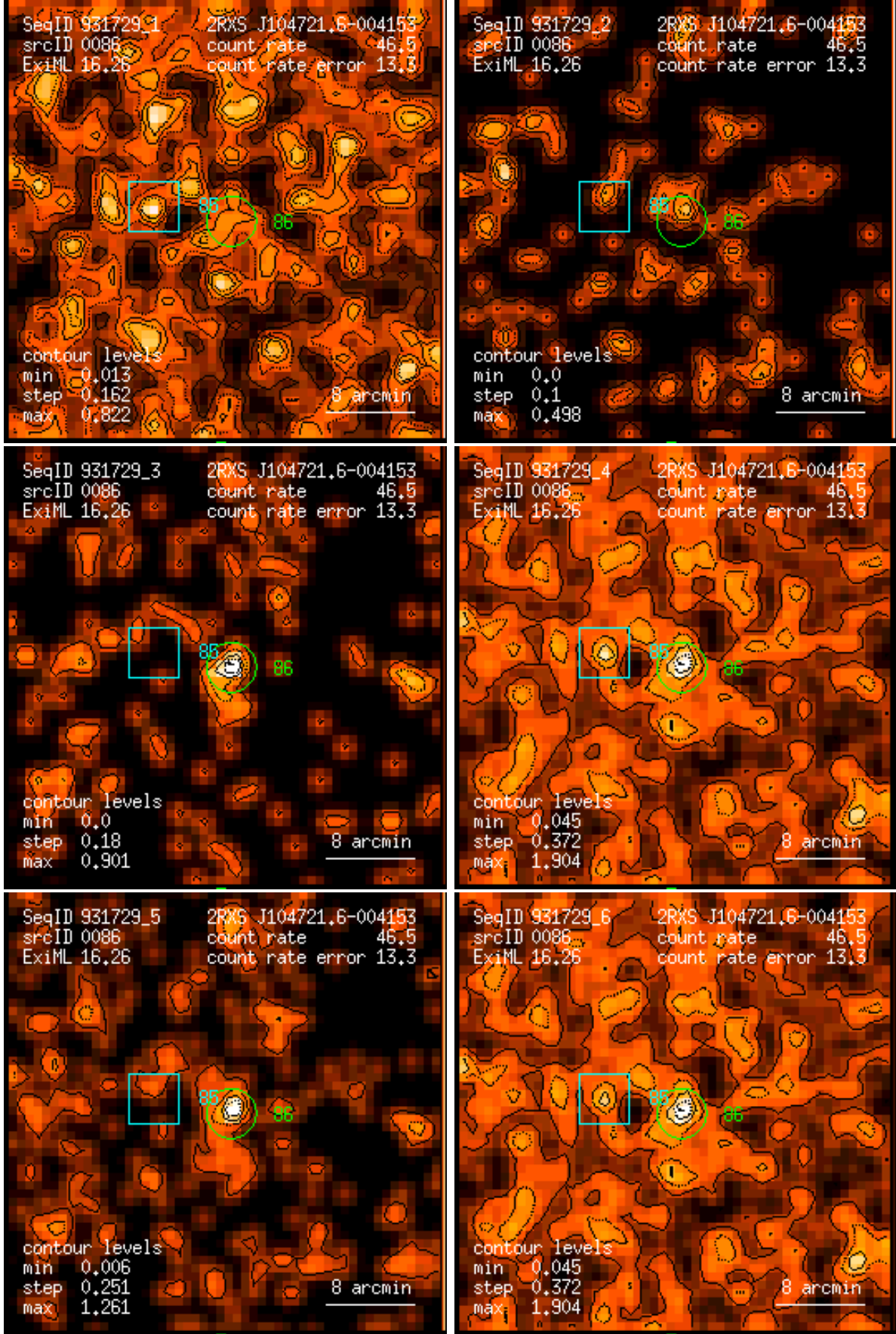
Figure 86: RASS 931729: detection 0086: band rate images, Gaussian filter: (1) PSPC channels 11 – 41, (2) 52 – 90, (3) 91 – 201, (4) 11 – 235, (5) 52 – 201, (6) 11 – 201. Broad band rates in counts/ks. Band rate contour levels in counts/ks/arcmin 2 .
